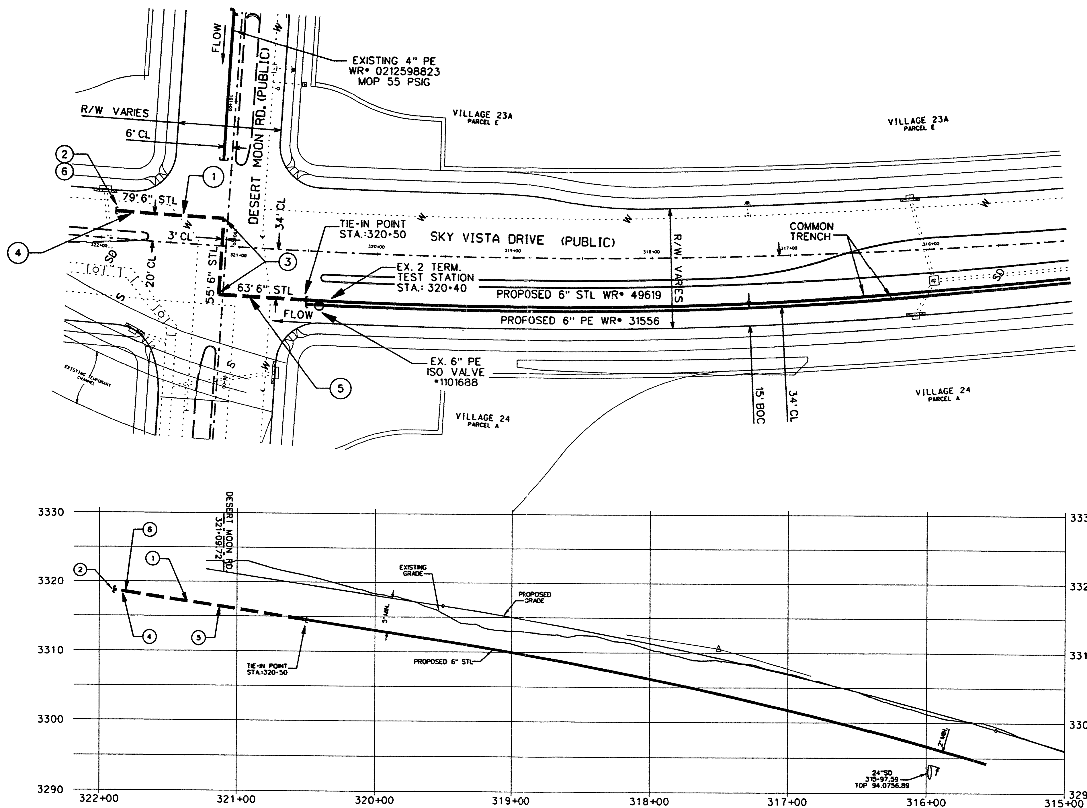
SKY VISTA DRIVE PROFILE SCALE: HORIZ. 1"=40' VERT. 1"=8'
