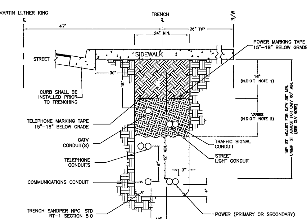
A SIDEWALK TRENCH DETAIL
