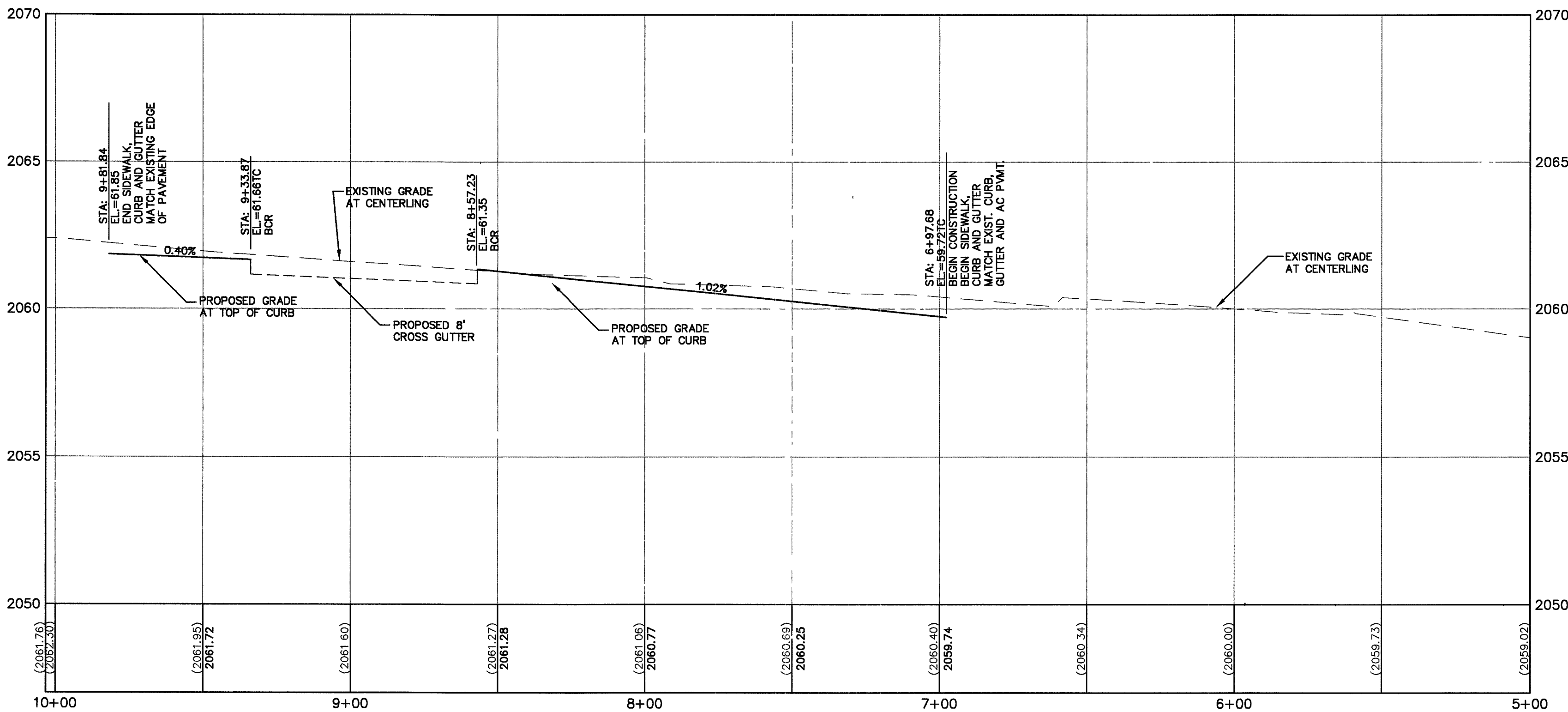
CAREY AVENUE - PROFILE
