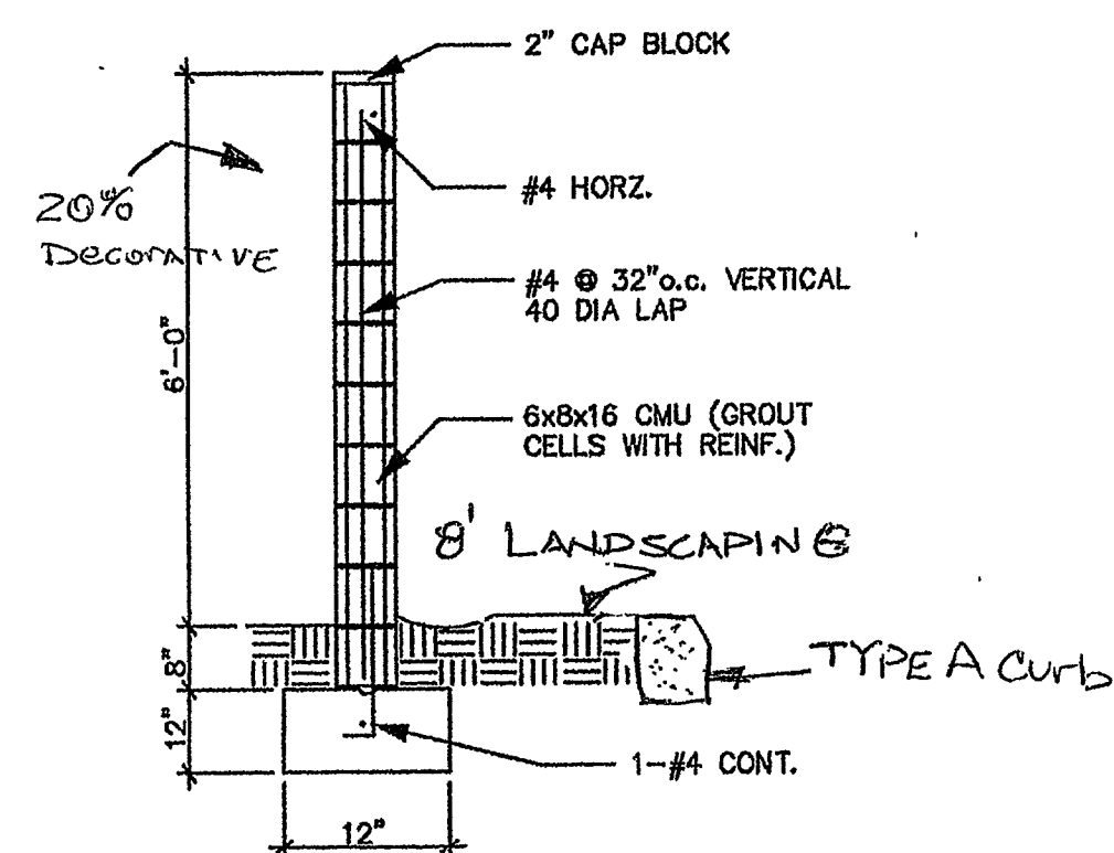
C PROPOSED PERIMETER WALL DETAIL SCALE: NOT TO SCALE
