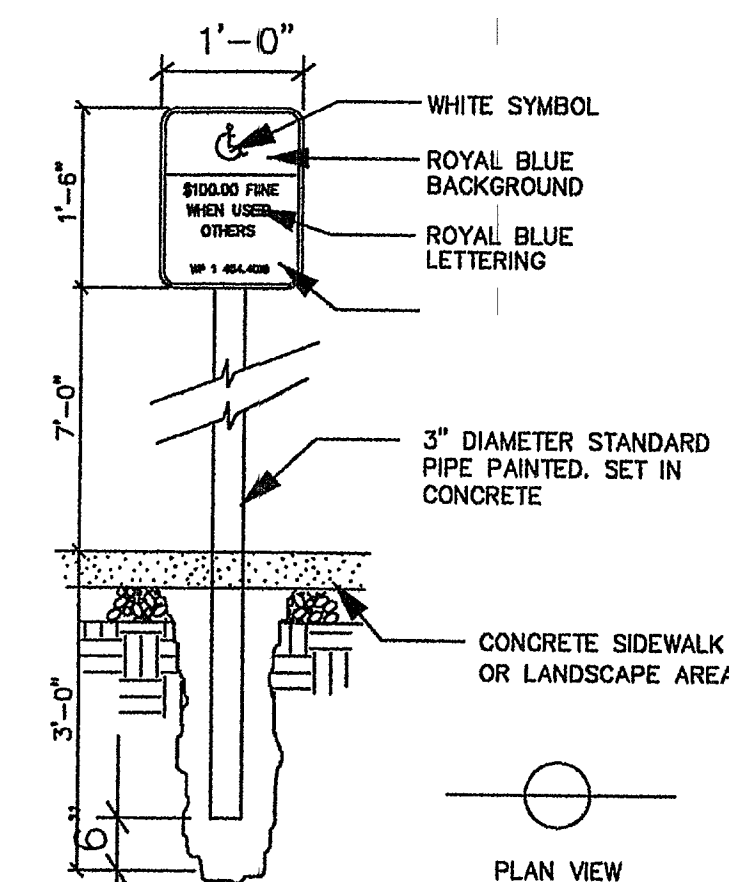
DISABLED PARKING SIGN SCALE: NOT TO SCALE
