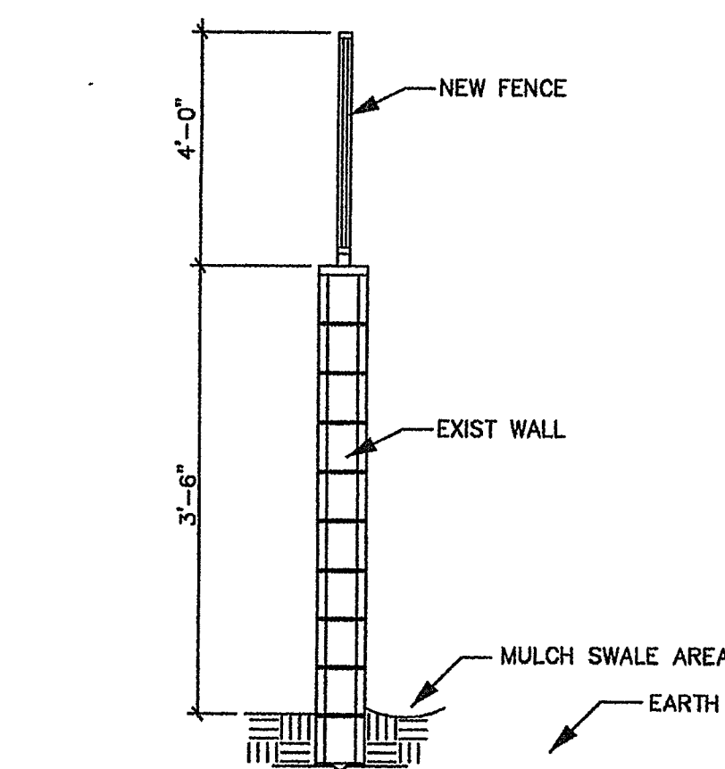
F FENCE ABOVE WALL DETAIL SCALE: NOT TO SCALE
