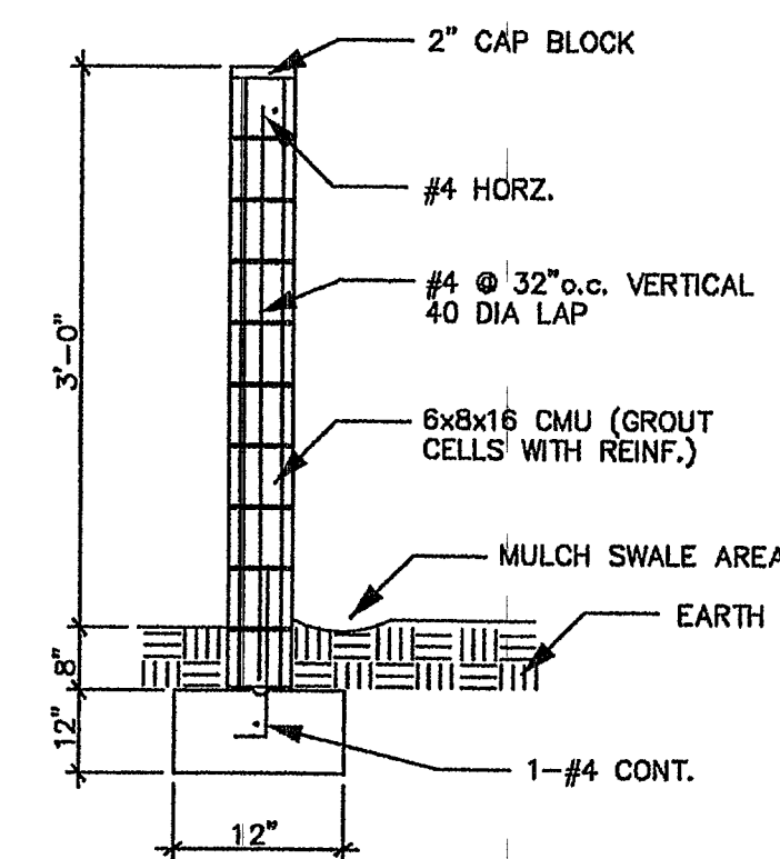
EXISTING PERIMETER WALL DETAIL SCALE: NOT TO SCALE
