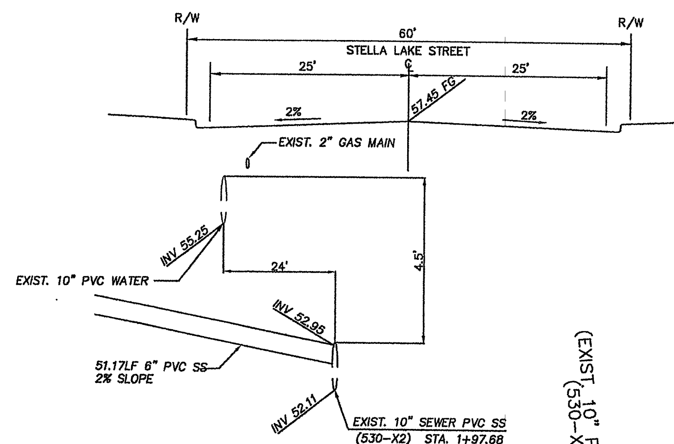
E SECTION DETAIL 1"=20'
