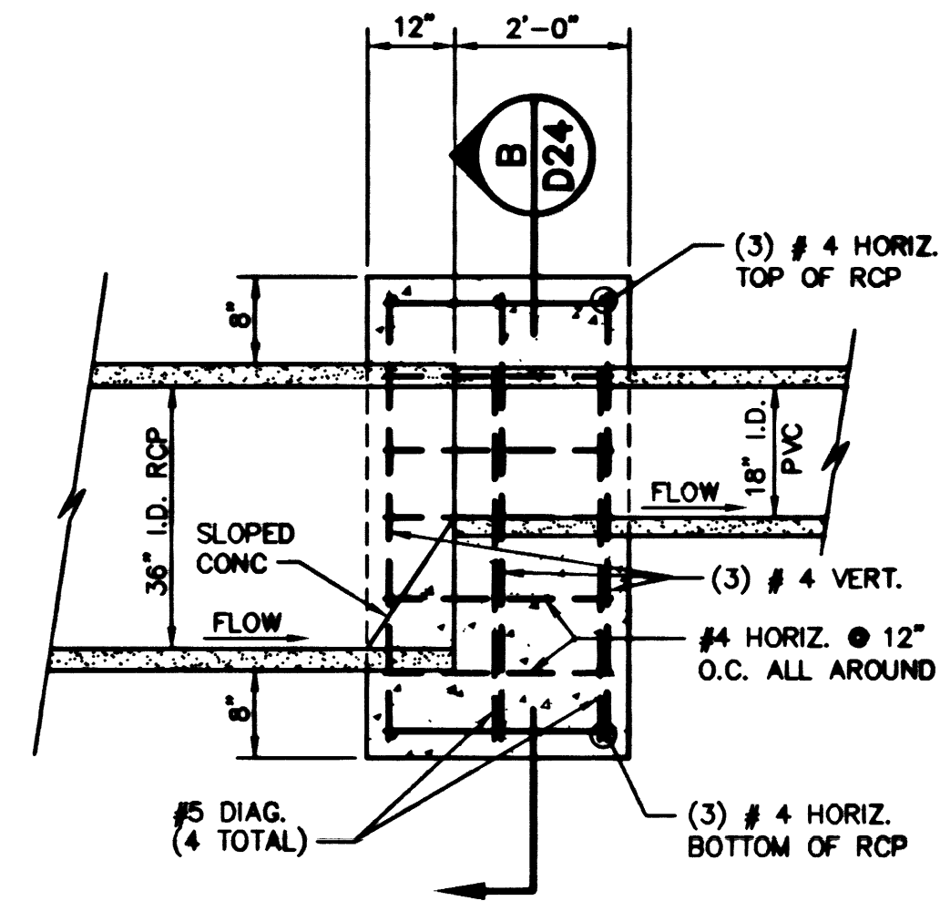
3 D24 36" RCP TO TEMPORARY 18" PVC CONNECTION AND PLUG DETAIL NO SCALE
