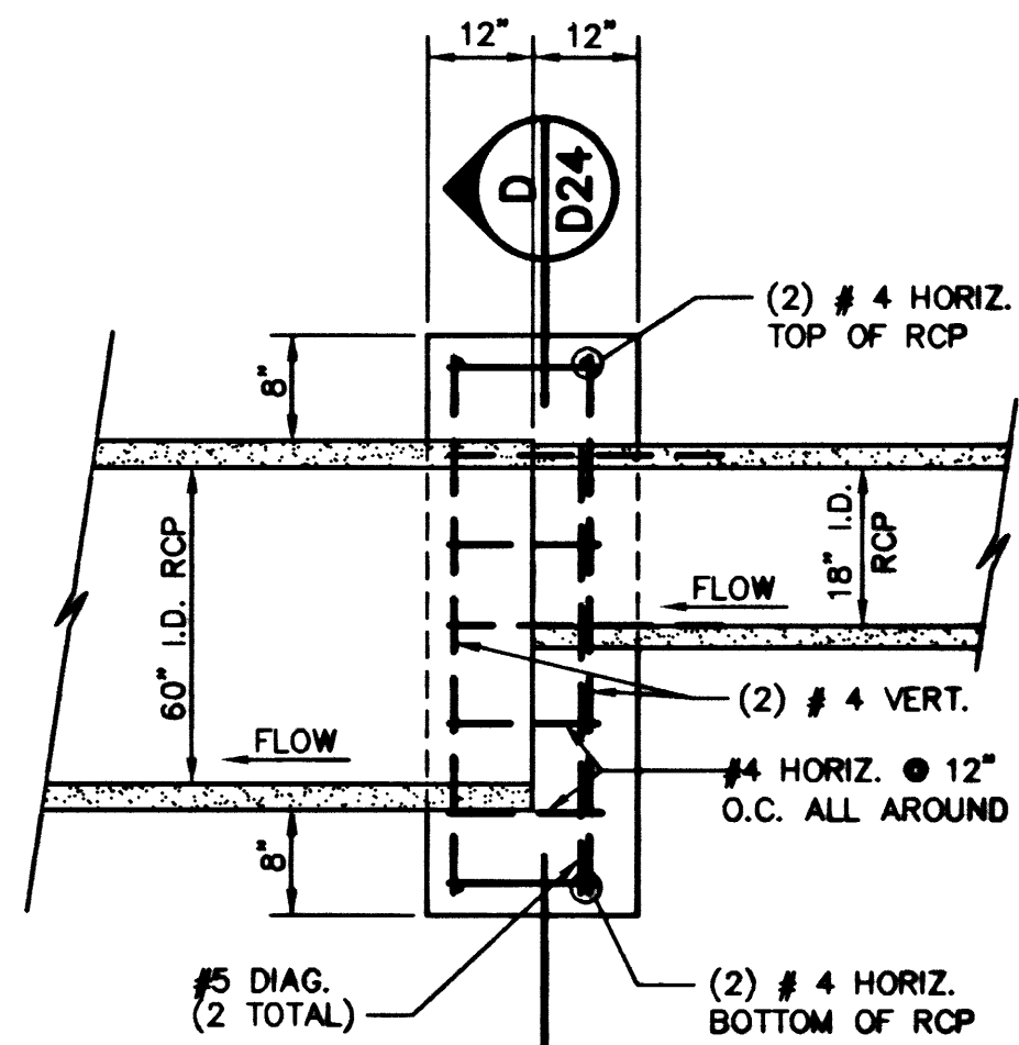
4 D24 60" RCP TO 18" RCP CONNECTION AND PLUG DETAIL NO SCALE
