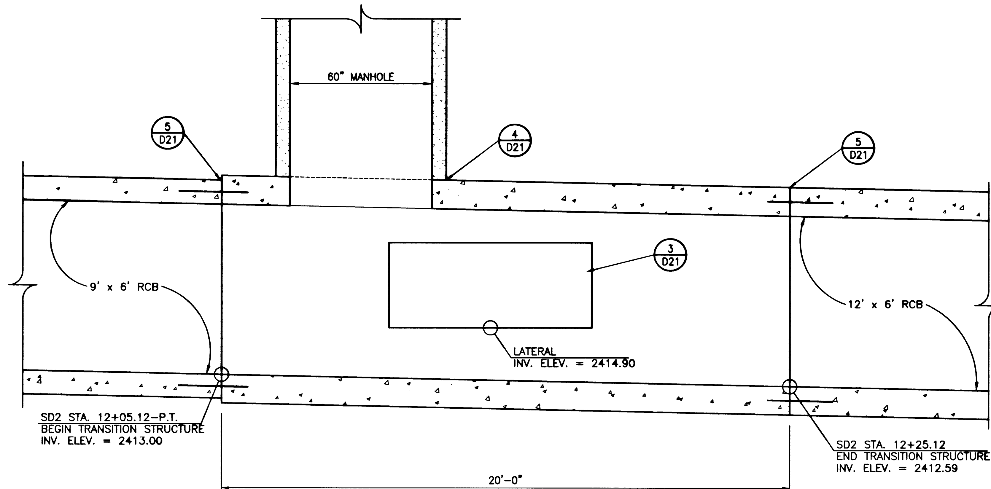
SECTION 1/2" = 1'-0"
