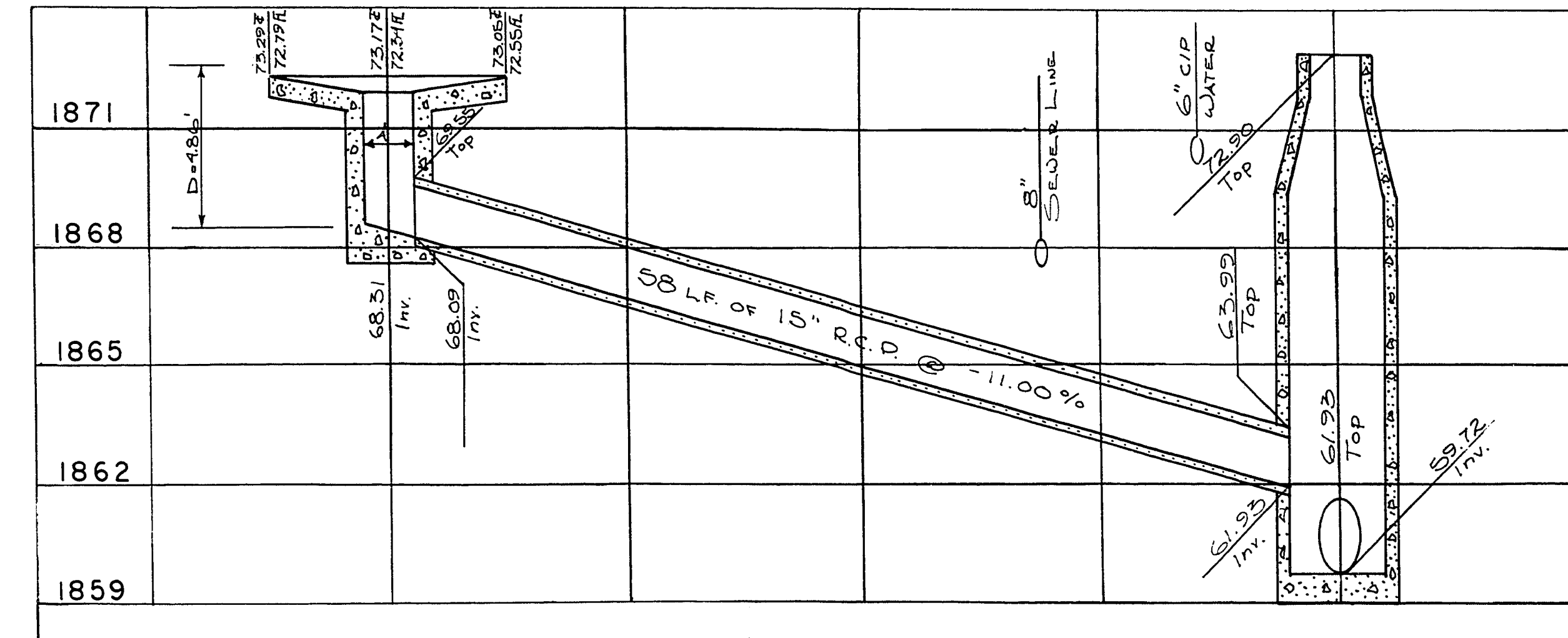
MANHOLE AND DROP INLET DETAIL AT PEYTON AND EASTERN
