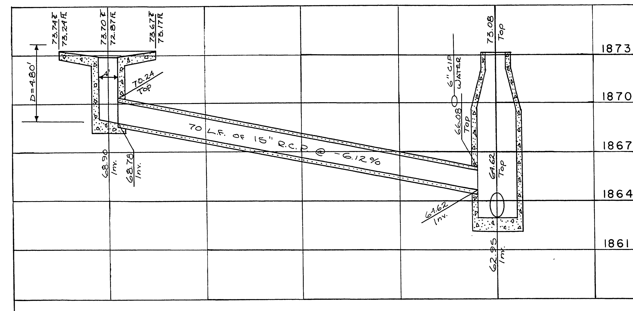
MANHOLE AND DROP INLET DETAIL AT WENGERT AND EASTERN
