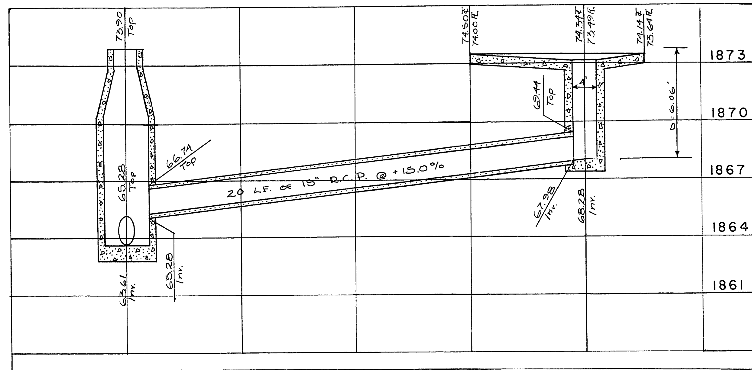
MANHOLE AND DROP INLET DETAIL AT SWEENEY AND EASTERN
