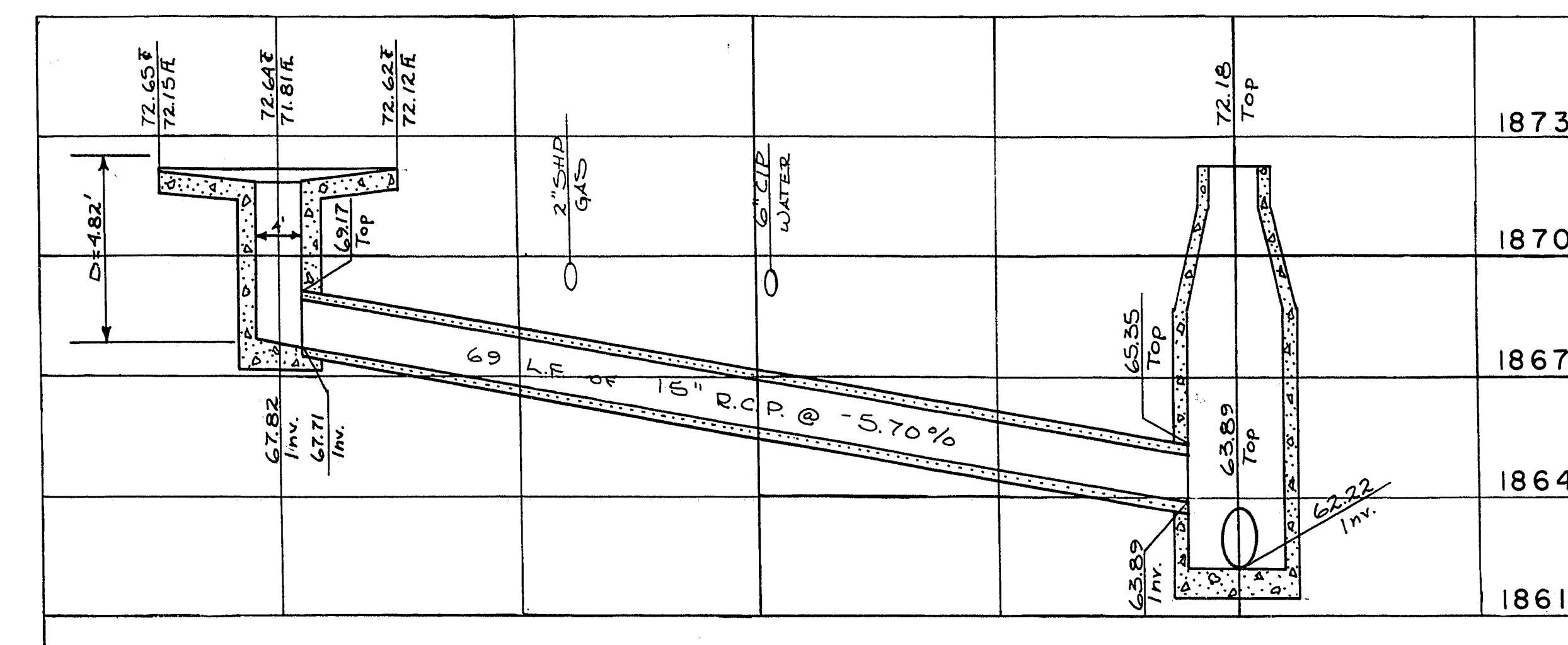
MANHOLE AND DROP INLET DETAIL AT FRANKLIN AND EASTERN
