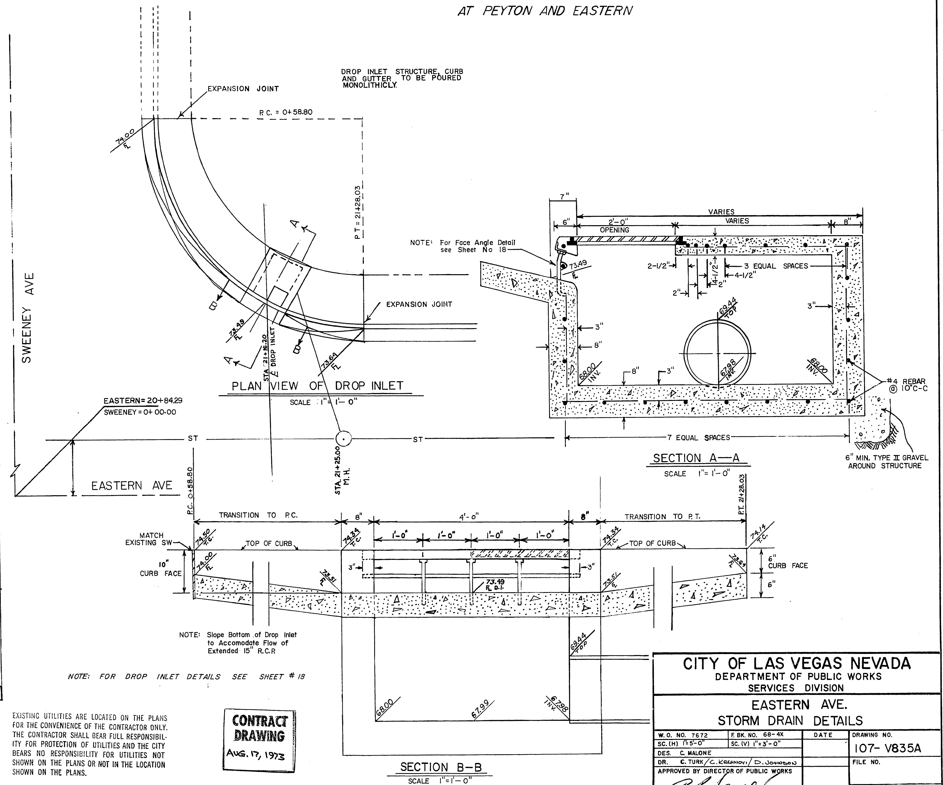
MANHOLE AND DROP INLET DETAIL AT PEYTON AND EASTERN
