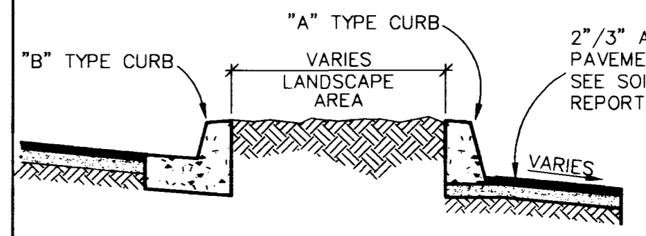
D TYPICAL ISLAND SECTION SCALE: NO SCALE
