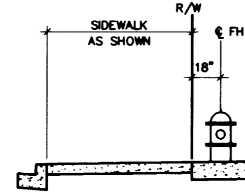
FIRE HYDRANT LOCATION DETAIL SCALE: NO SCALE
