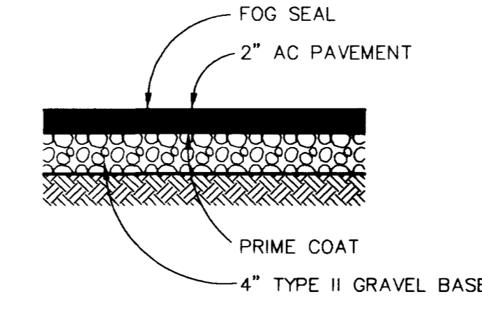
TYP. ONSITE A.C. PAVEMENT SECTION SCALE: NO SCALE
