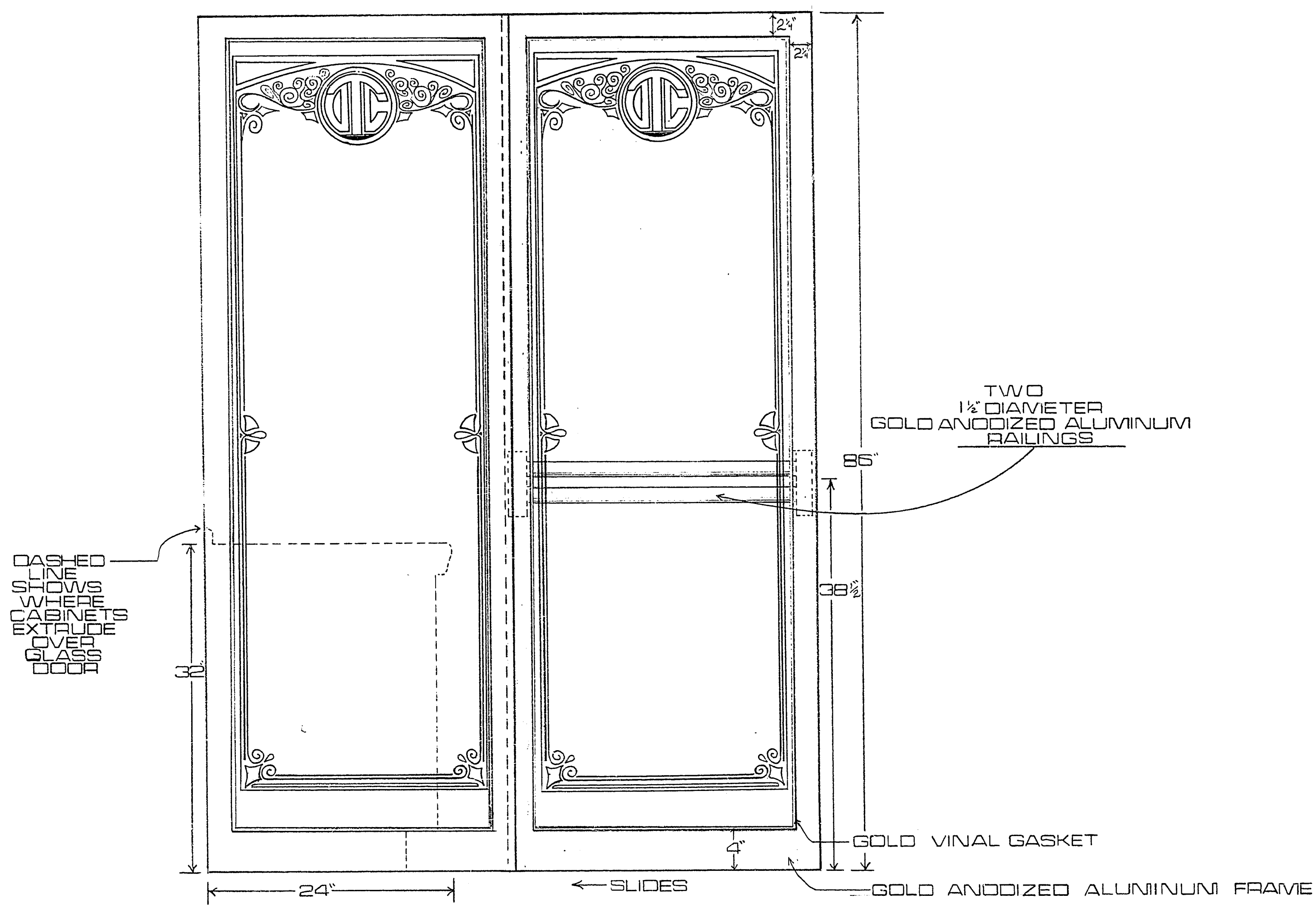
ELEVATION OF SLIDING GLASS DOOR WITH ETCHED GLASS PATTERNS (ELEVATION FROM BUS TICKET SIDE) SCALE 1/2" = 1' FOR DOWNTOWN TRANSPORTATION CENTER INTERIOR
