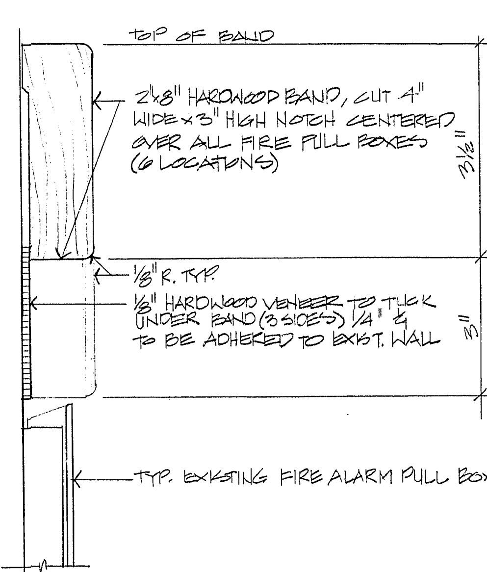
BAND AT FIRE PULL BOXES
