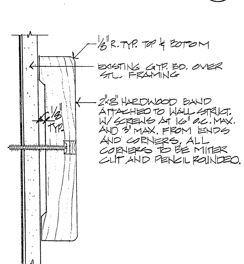
JAMB AND CORNER DETAIL
