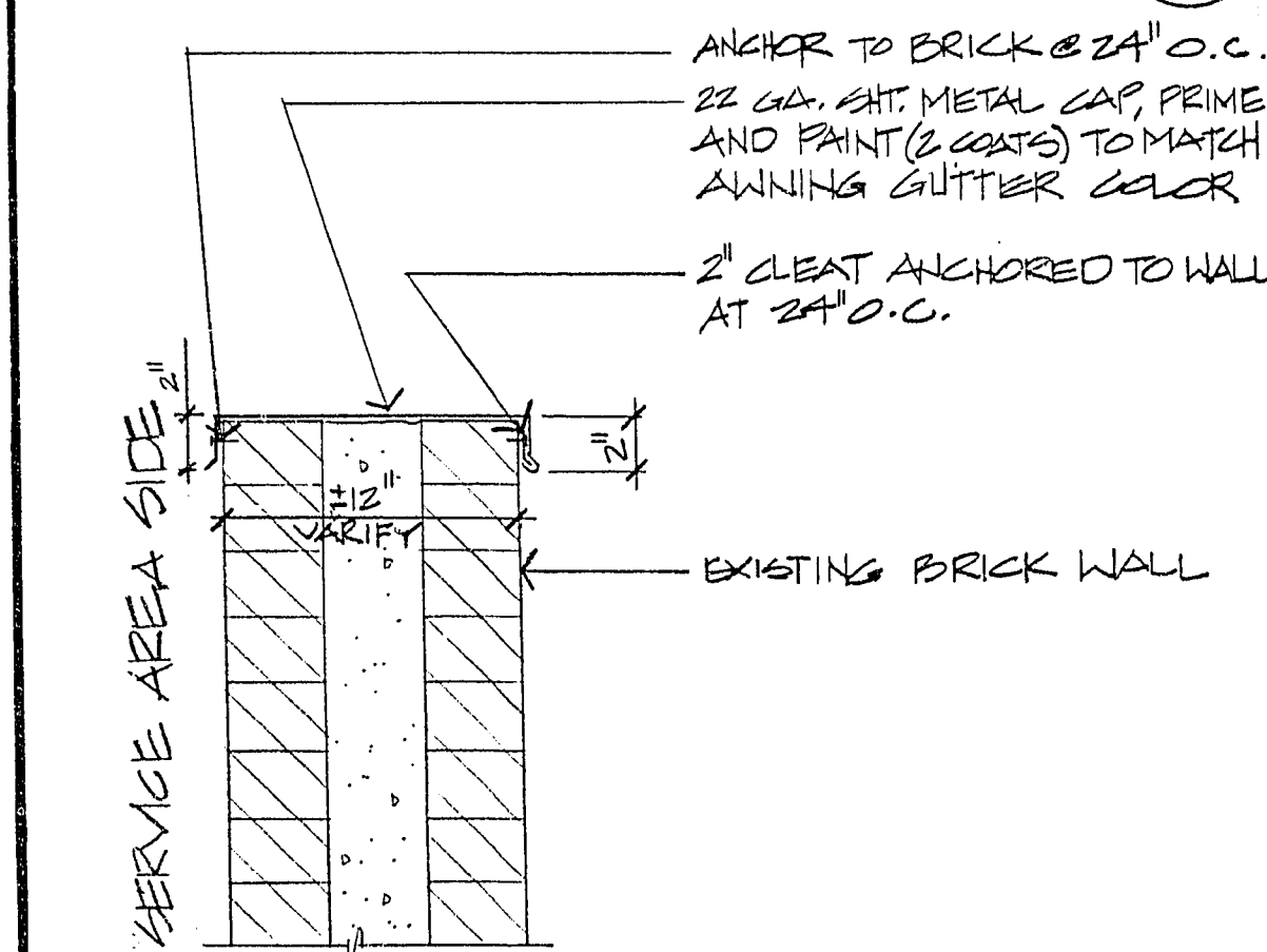
SILL DETAIL
