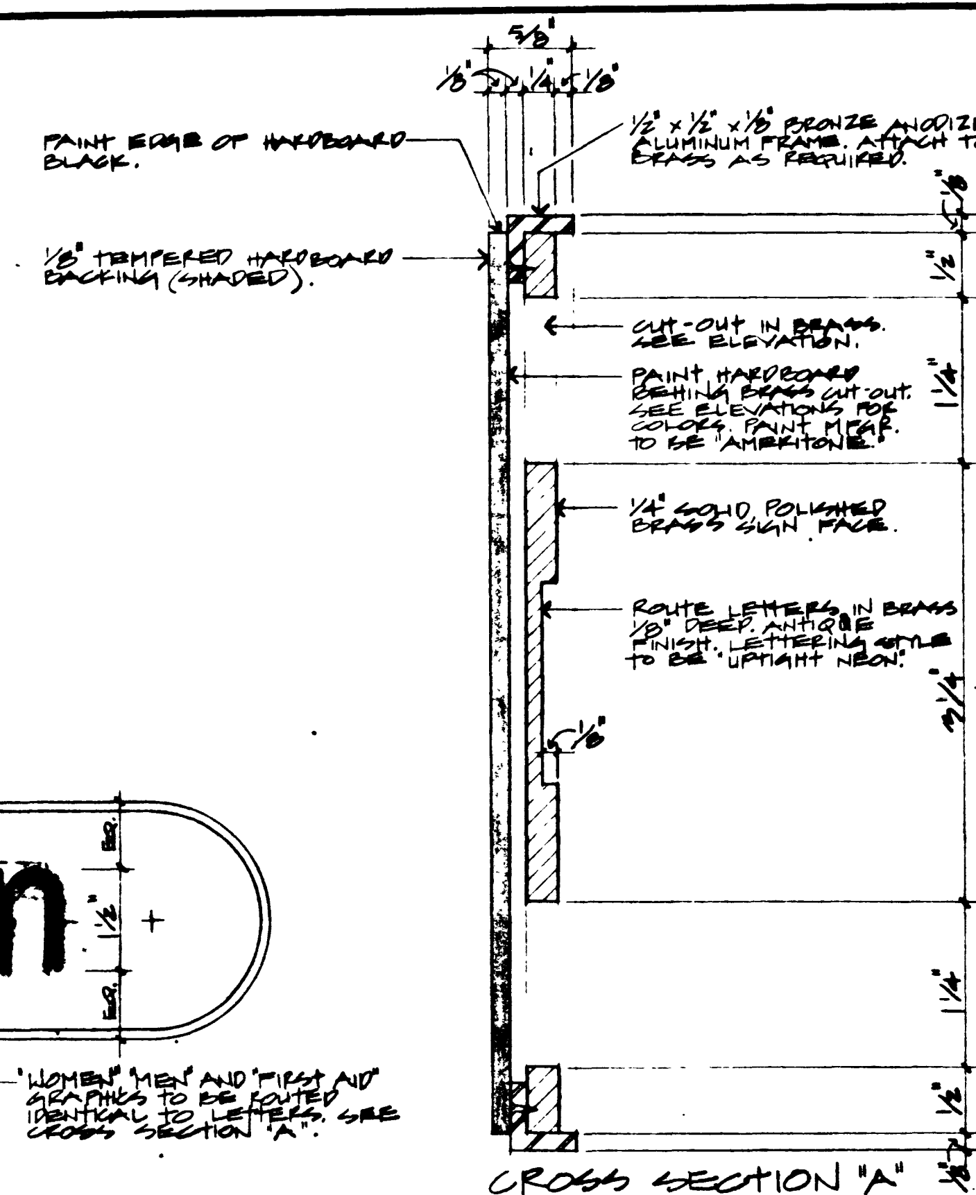
CROSS SECTION "A"
