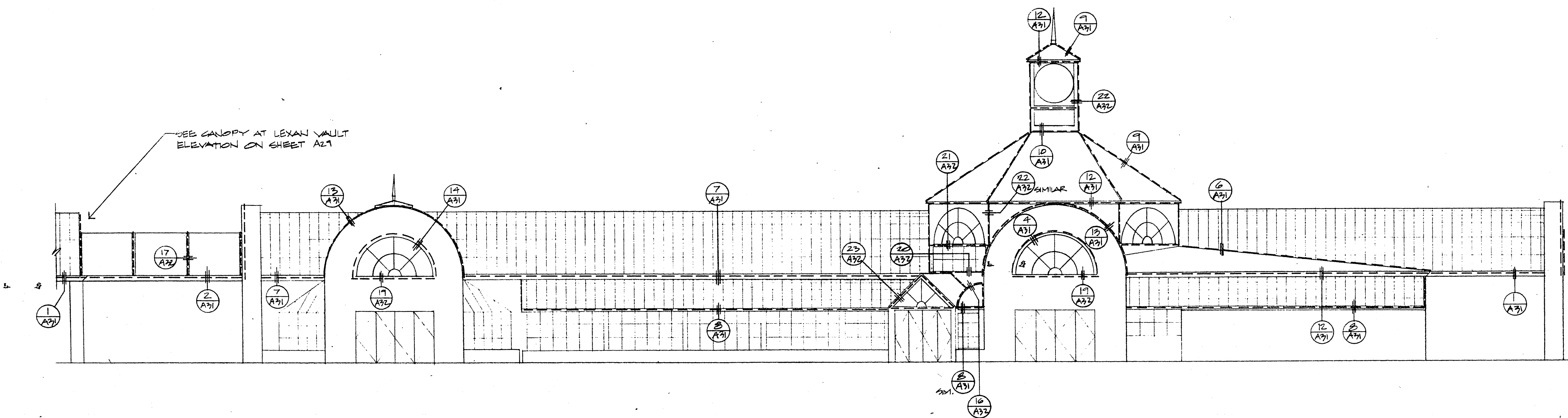
EAST ELEVATION 3/8" = 1'-0"
