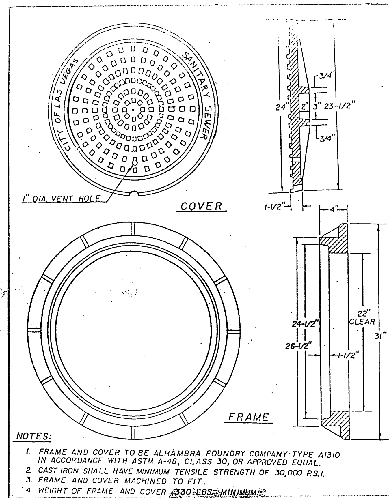
MANHOLE COVER & RING
