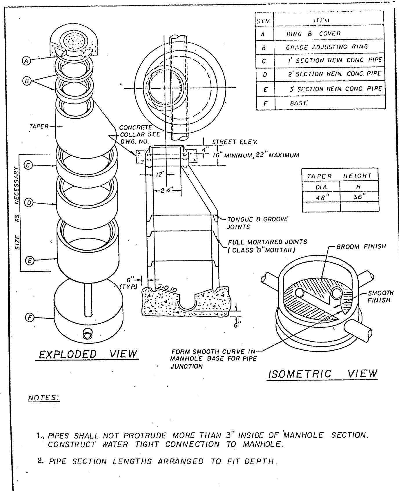
ECCENTRIC MANHOLE
