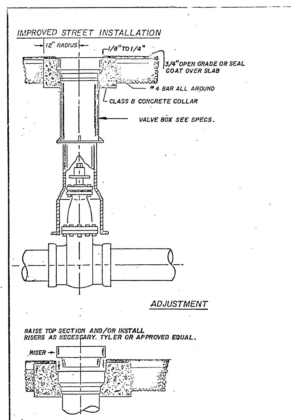
VALVE BOX ADJUSTMENT
