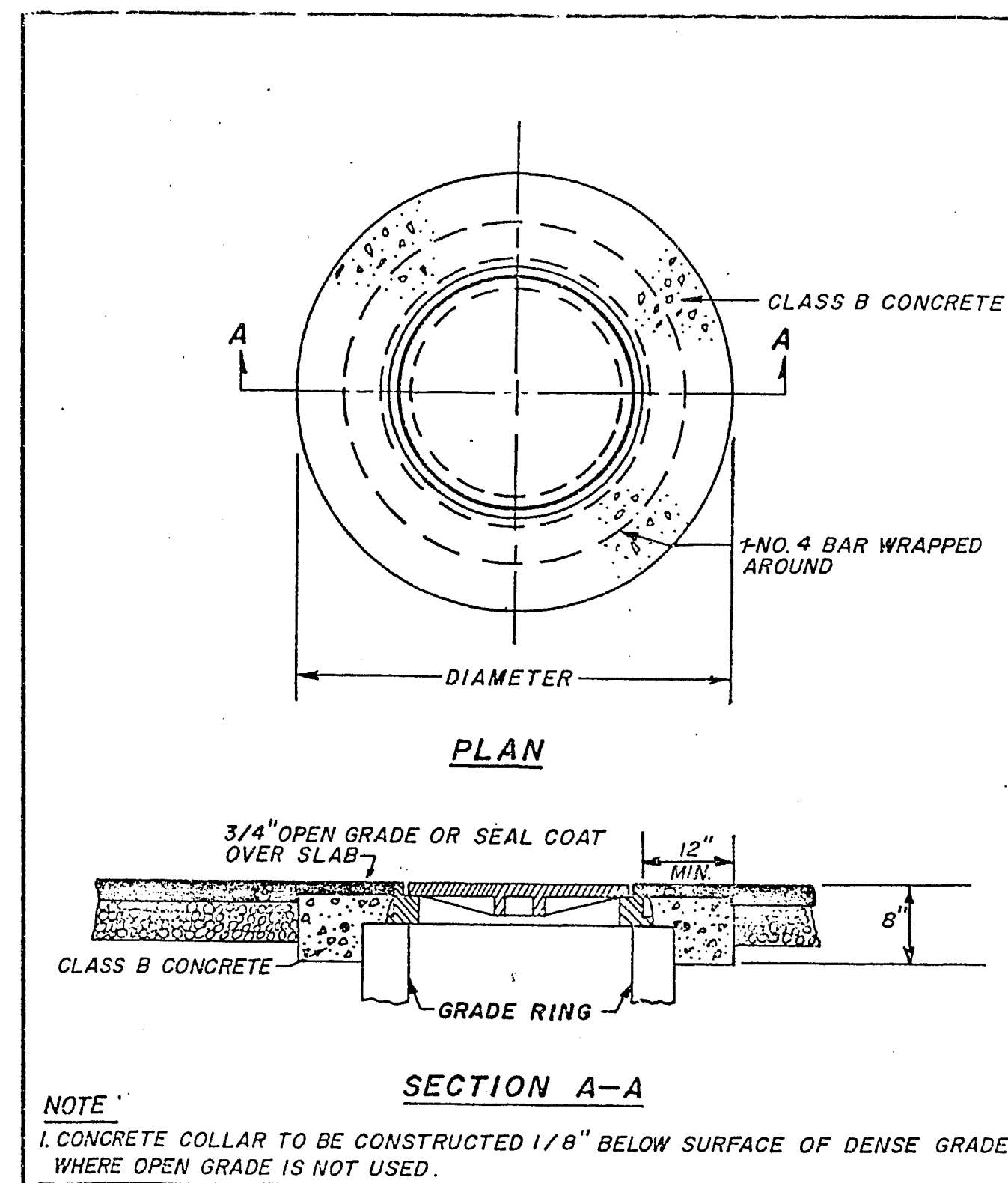
CONCRETE COLLAR AROUND MANHOLES
