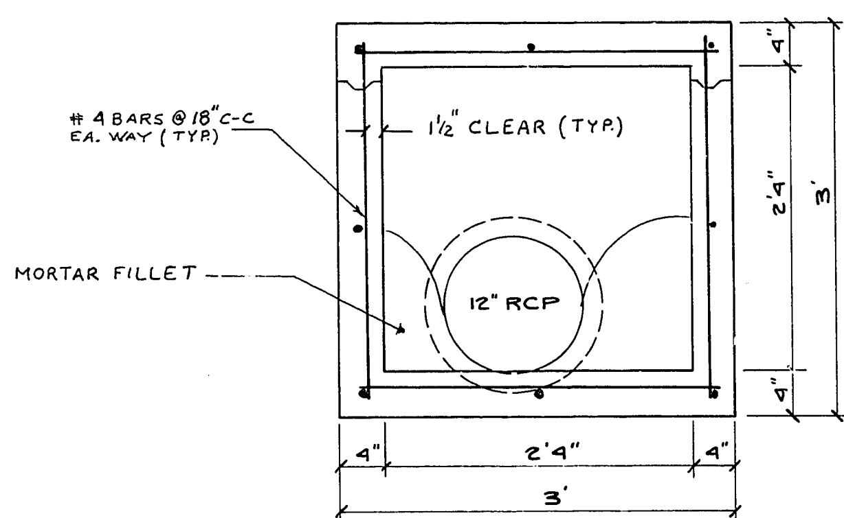
SECTION C SCALE 1"=1'-0"
