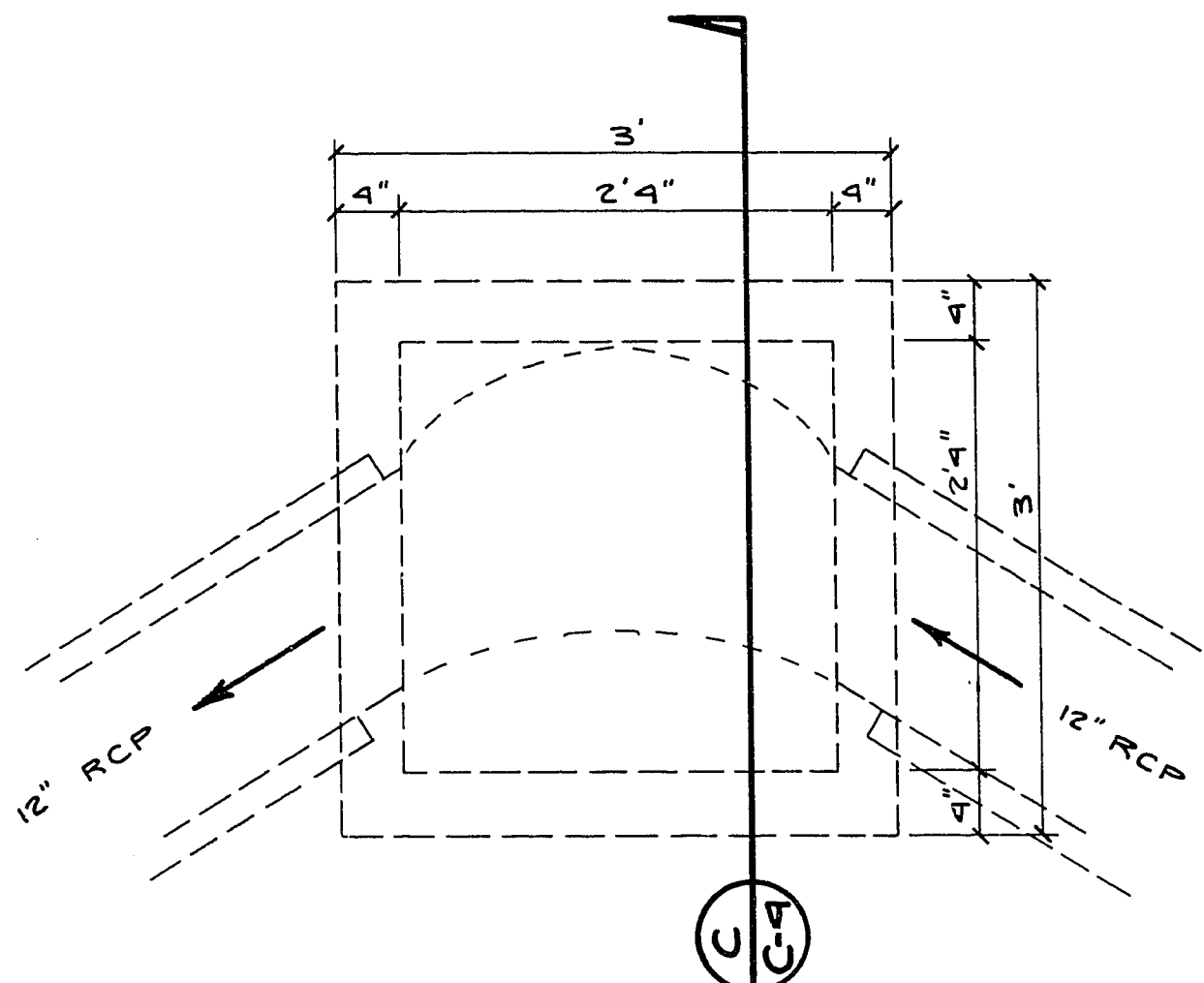
DETAIL 7 SCALE 1"=1'-0"
