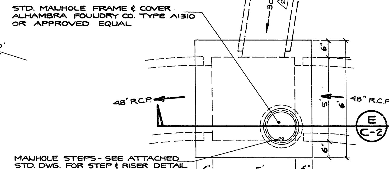
DETAIL 8 SCALE 1"=3'-0" JUNCTION BOX
