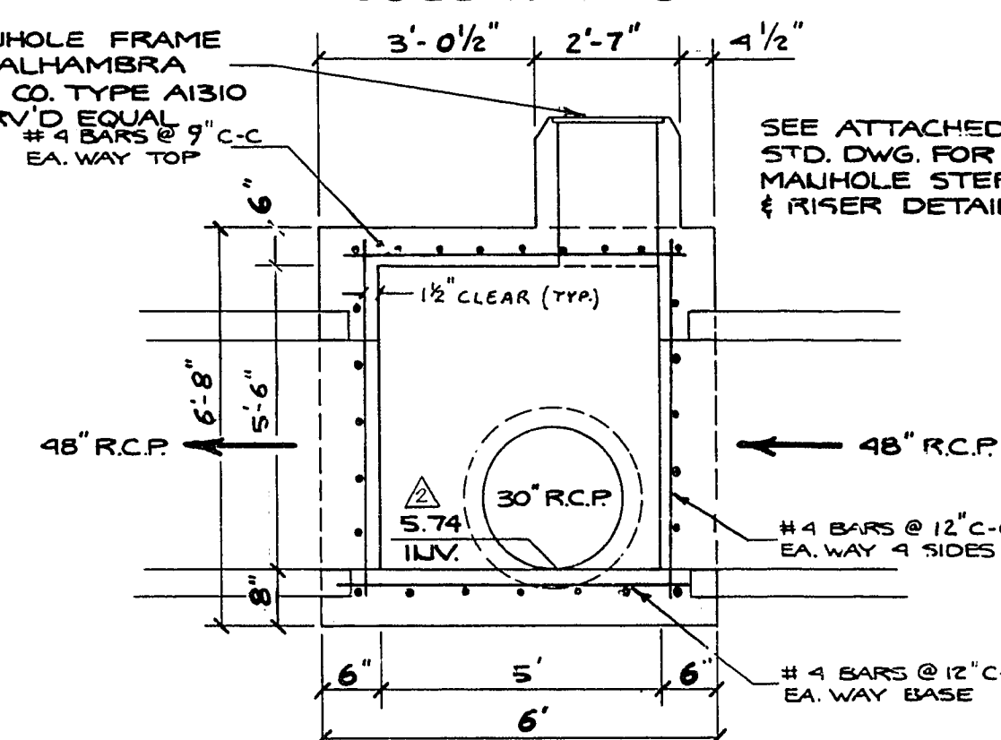
DETAIL 8 SCALE 1"=3'-0" JUNCTION BOX
