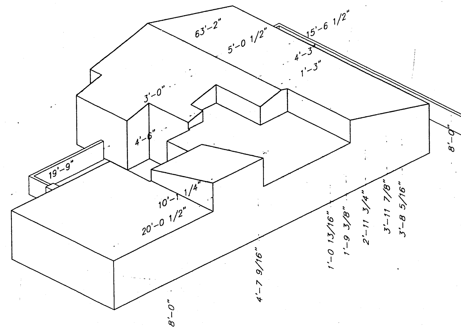
DUPLEX A UNIT RIGHT OBLIQUE VIEW SCALE: 1/8" = 1'
