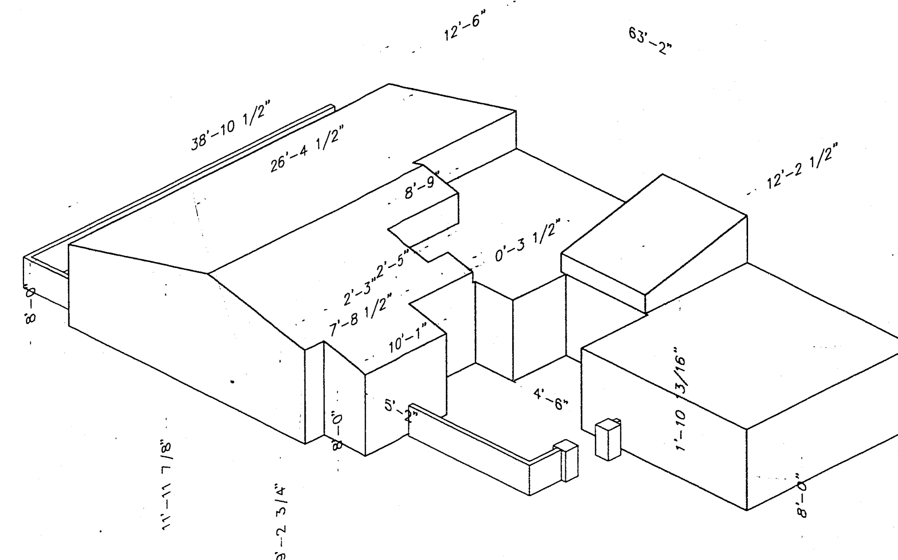
DUPLEX A UNIT LEFT OBLIQUE VIEW SCALE: 1/8" = 1'
