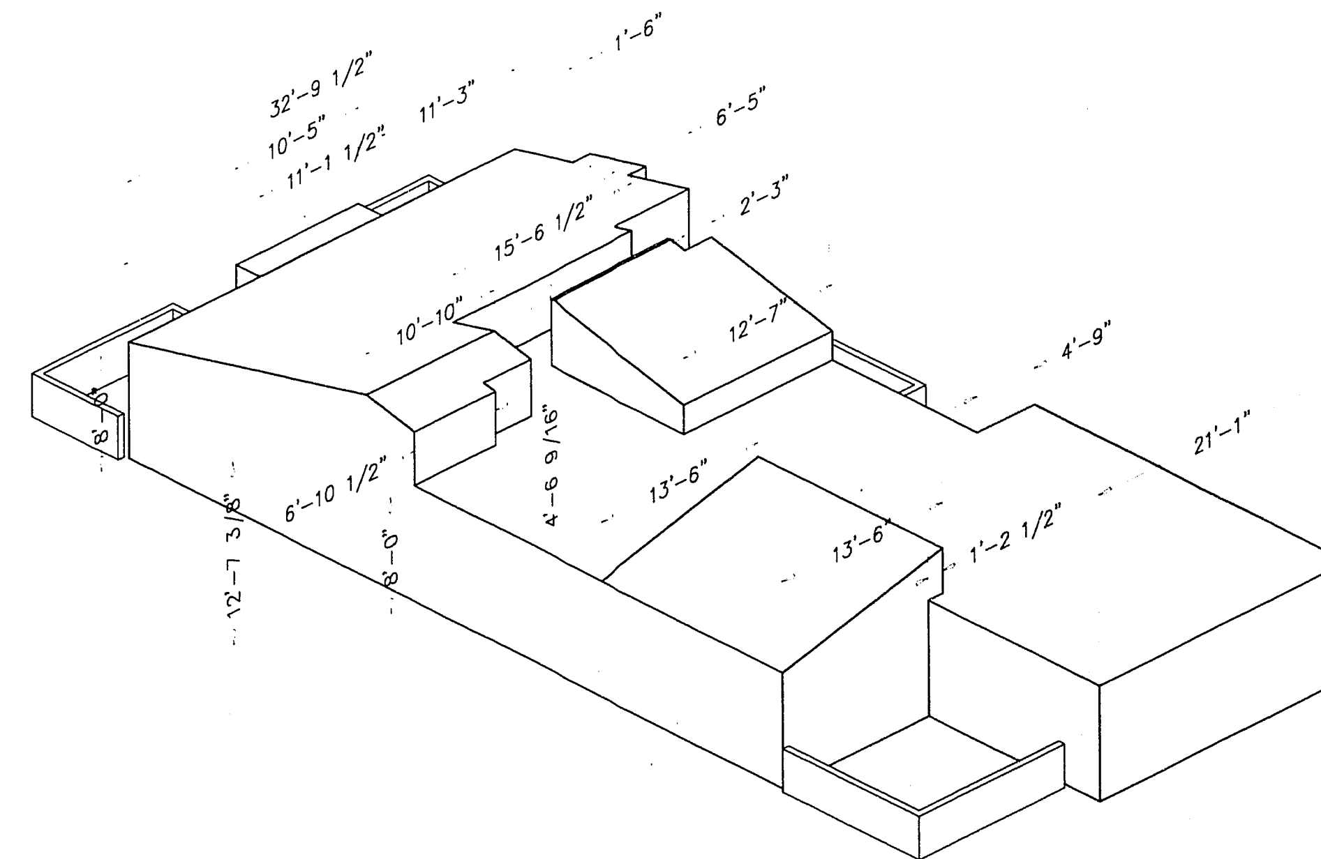
TRIPLEX C UNIT LEFT OBLIQUE VIEW SCALE: 1/8" = 1'
