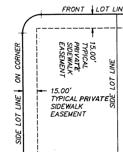
TYP. PRIVATE SIDEWALK EASEMENT LOCATION
