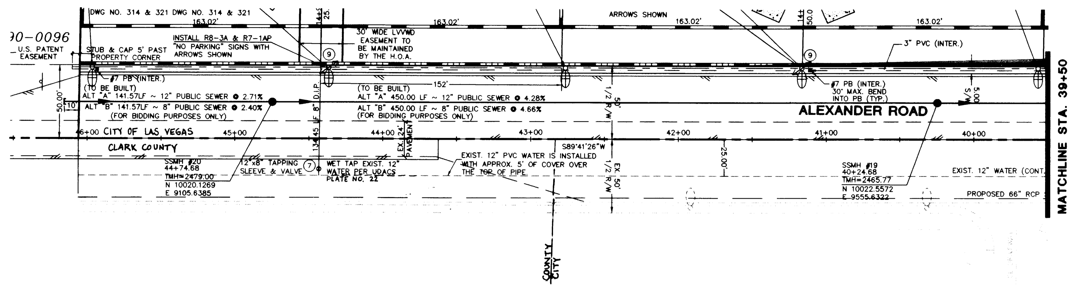
ALEXANDER ROAD (PUBLIC) SCALE: 1"=40' HORIZ. 1"=4' VERT.
