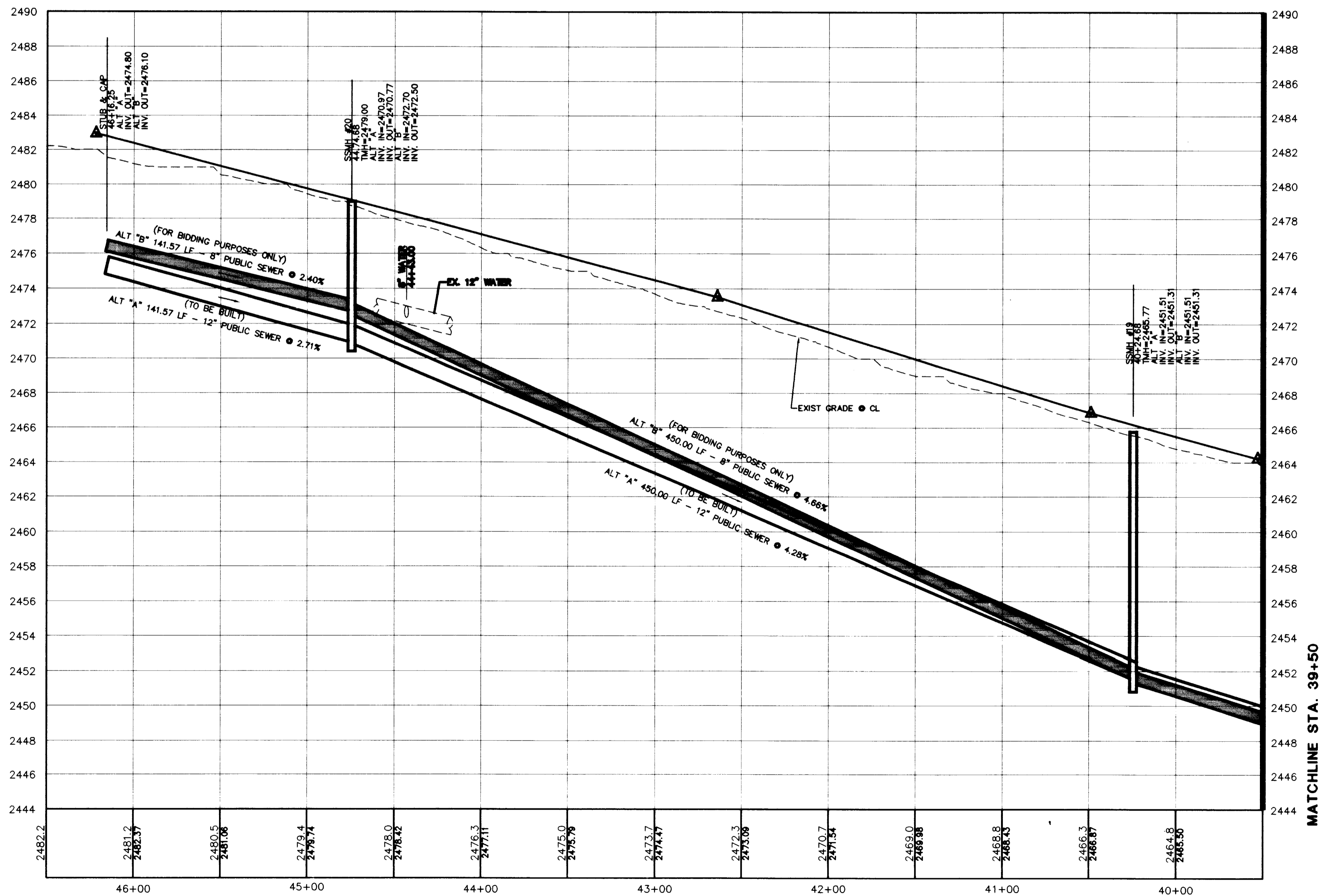
ALEXANDER ROAD (PUBLIC) SCALE: 1"=40' HORIZ. 1"=4' VERT.
