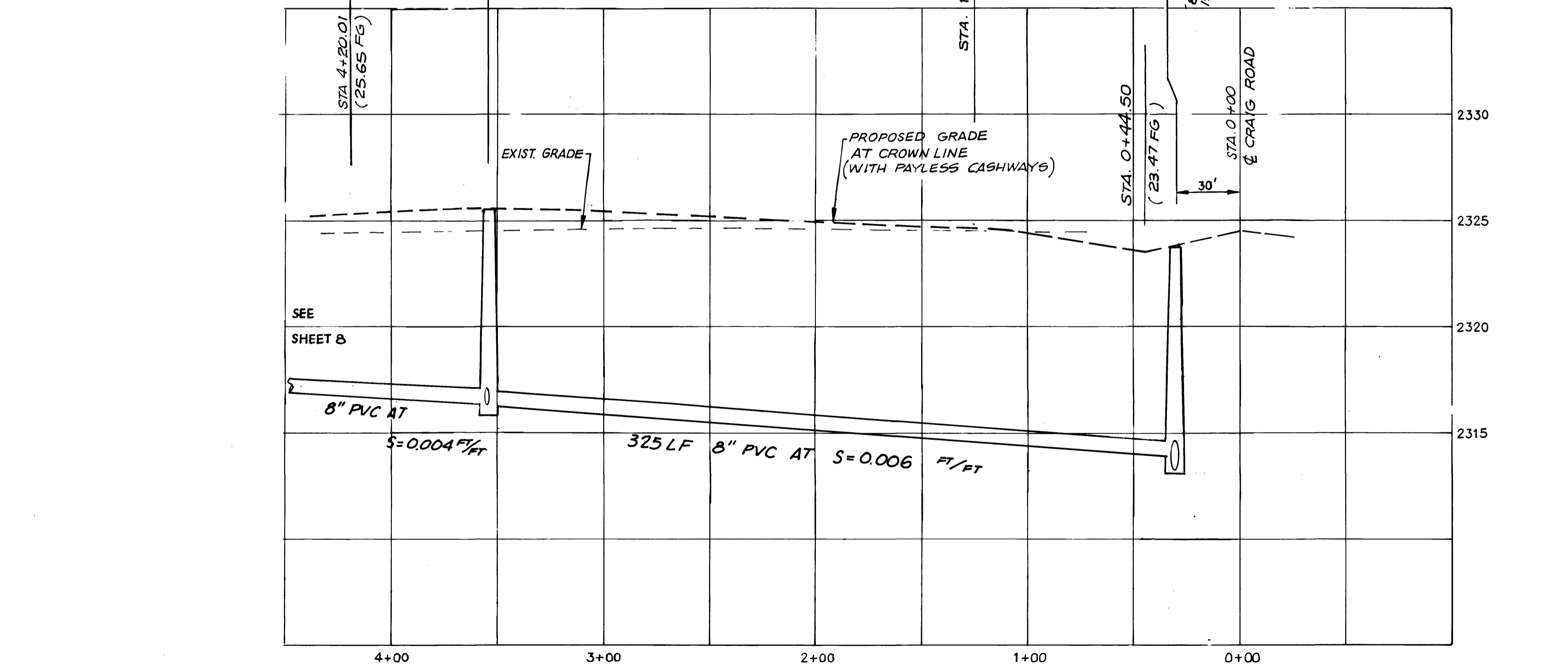
PROFILE SCALE: 1" = 40' HORIZ. 1" = 4' VERT.
