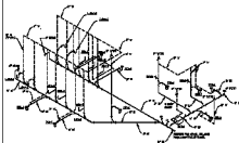
1 WASTE ISOMETRIC NOT TO SCALE
