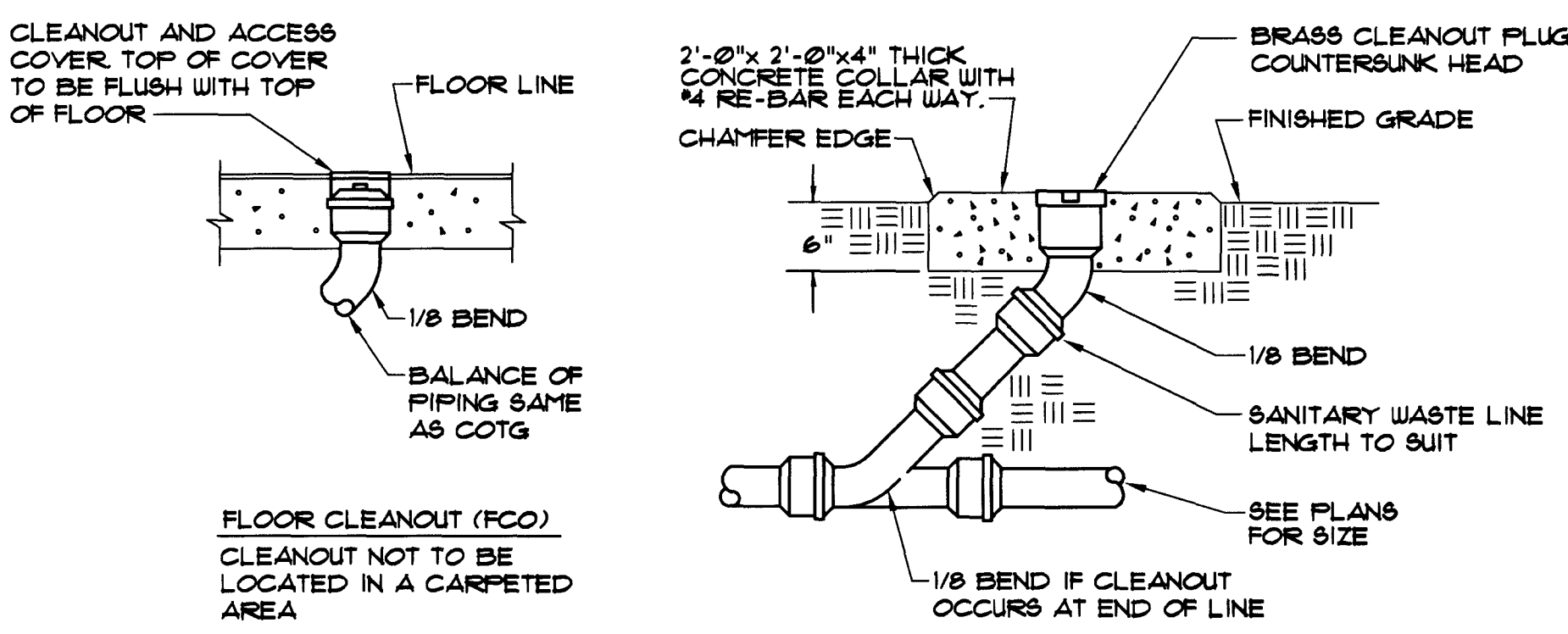
GRADE CLEANOUT (GCO)
