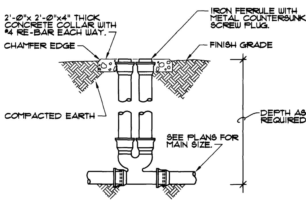
TWO-WAY GRADE CLEANOUT
