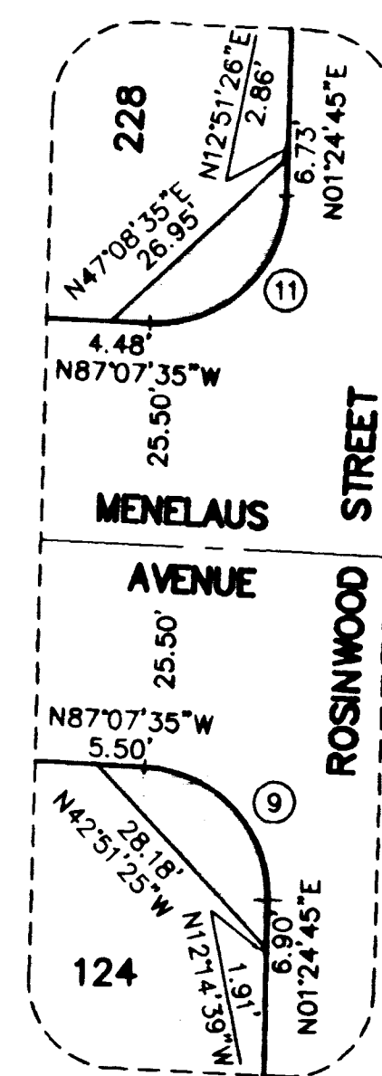
DETAIL 'C' NOT TO SCALE
