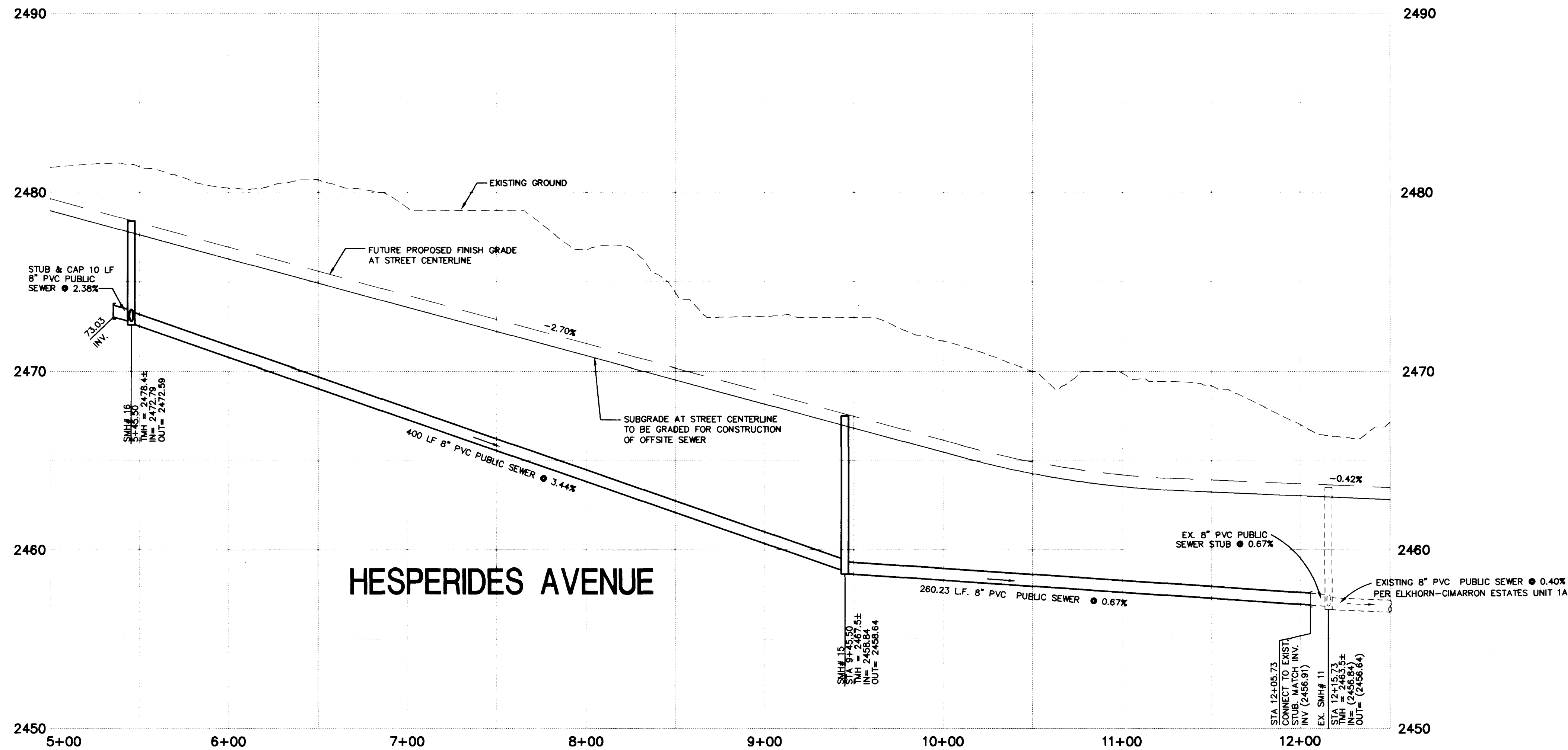
PROFILE SCALE: HORIZ. 1" = 40' VERT. 1" = 4' OFFSITE SEWER
