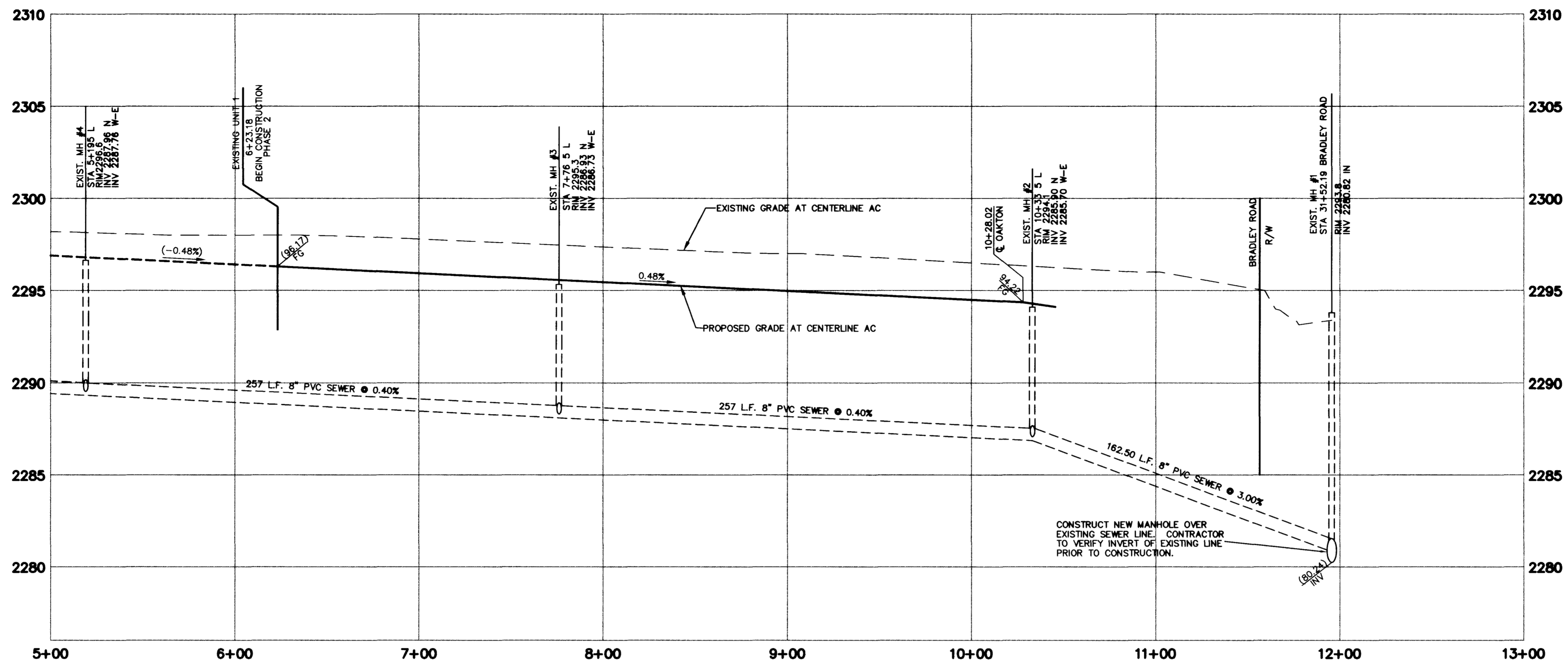
PROFILE SCALE: HORIZ. 1" = 40' VERT. 1" = 4'
