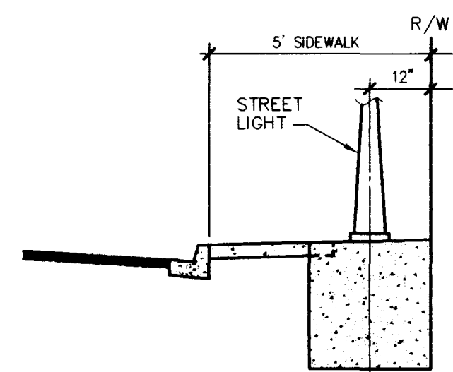
TYPICAL STREET LIGHT LOCATION DETAIL
