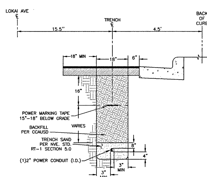
TRENCH DETAIL 1-2" CONDUIT SECTION "B"
