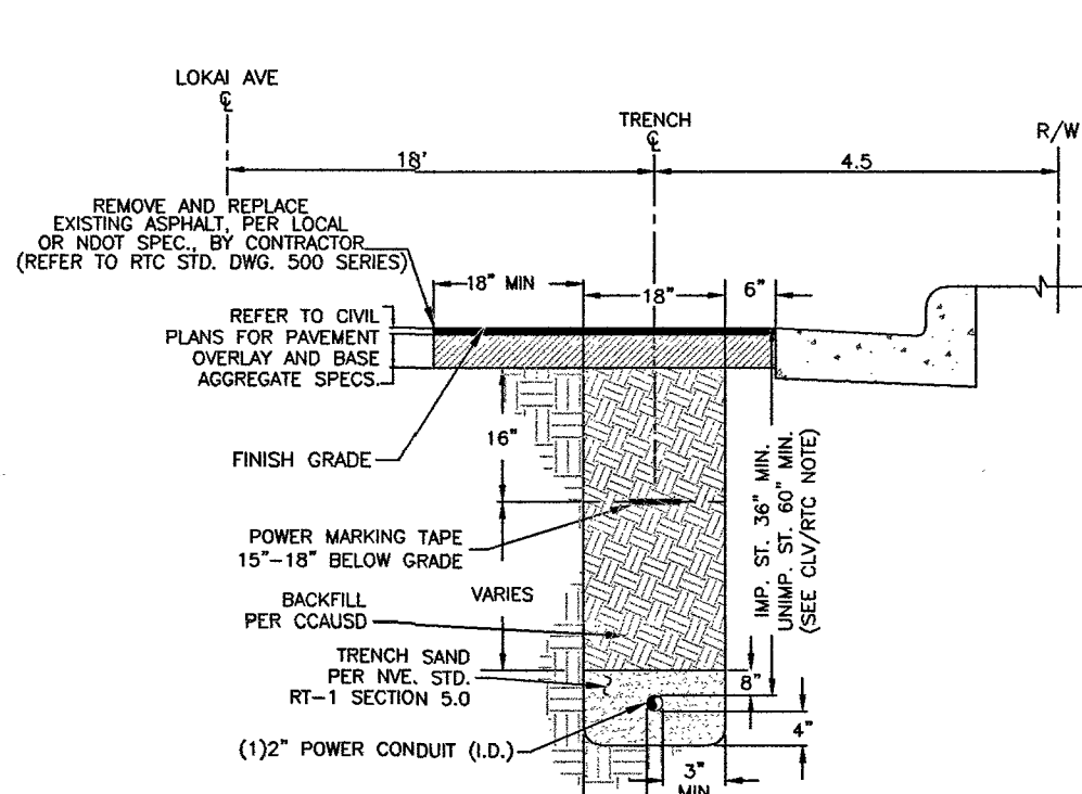
TRENCH DETAIL SECTION "C"
