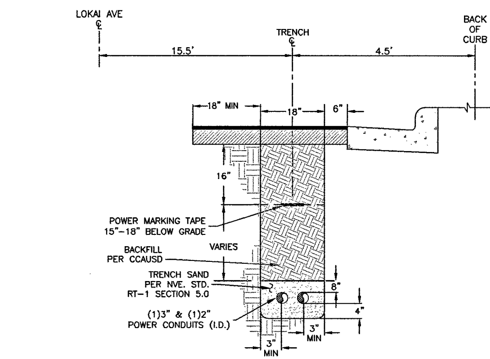
TRENCH DETAIL (1)3" & (1)2" POWER CONDUIT (I.D.) SECTION "A"
