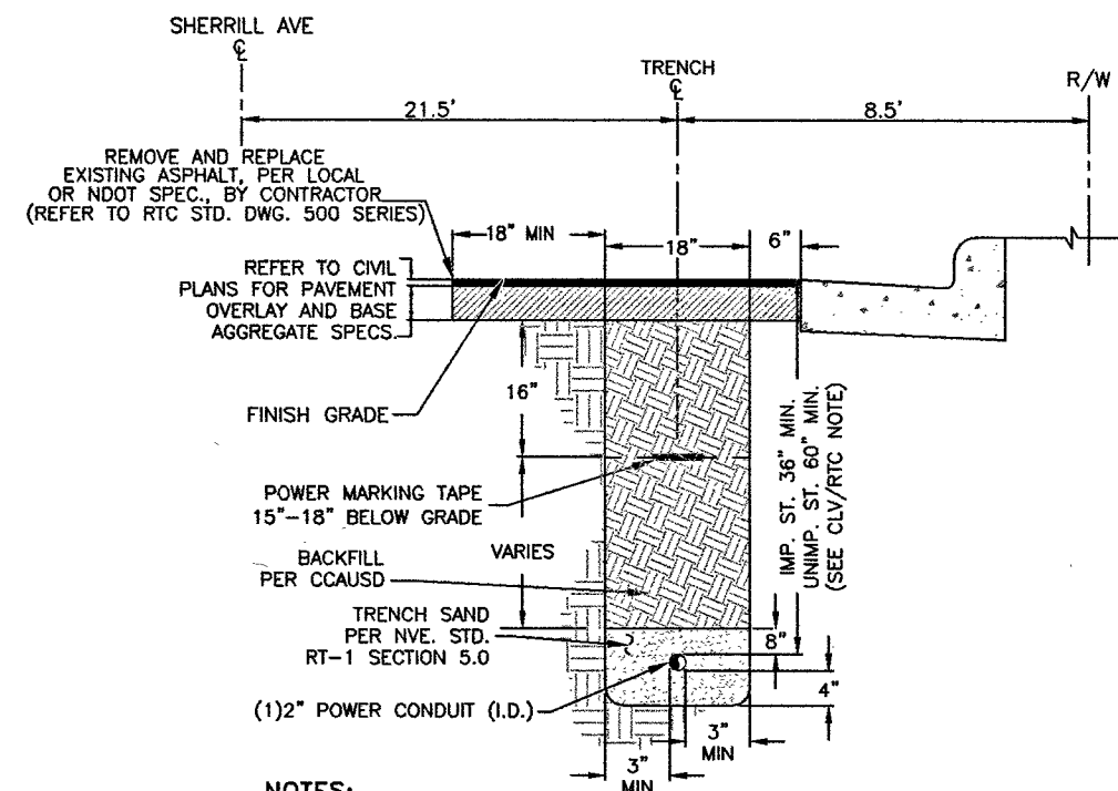
TRENCH DETAIL 1-2" CONDUIT SECTION "A"
