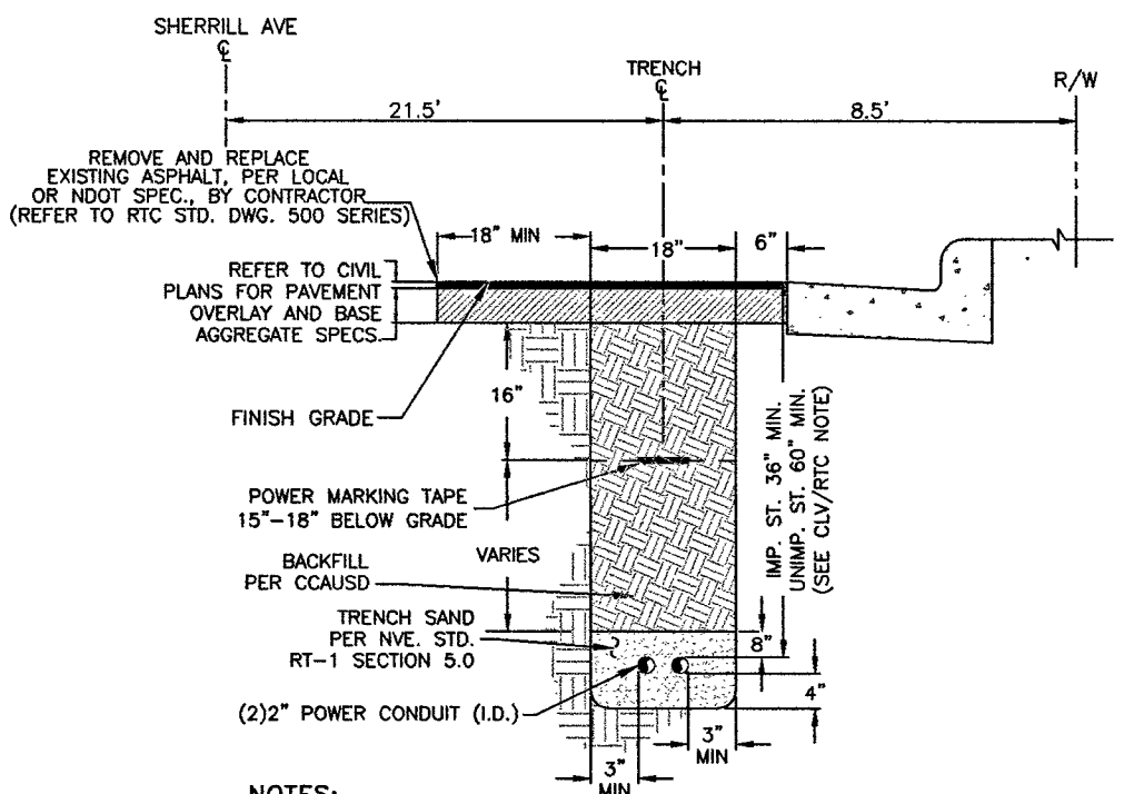
TRENCH DETAIL 1-2" CONDUIT SECTION "B"
