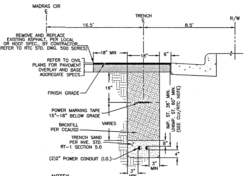
TRENCH DETAIL 1-2" CONDUIT SECTION "C"
