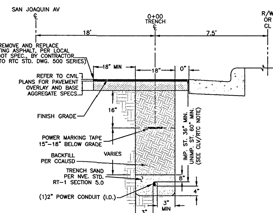
TRENCH DETAIL SECTION "B"
