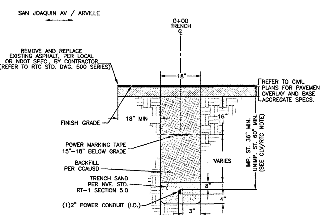
TRENCH DETAIL SECTION "C"
