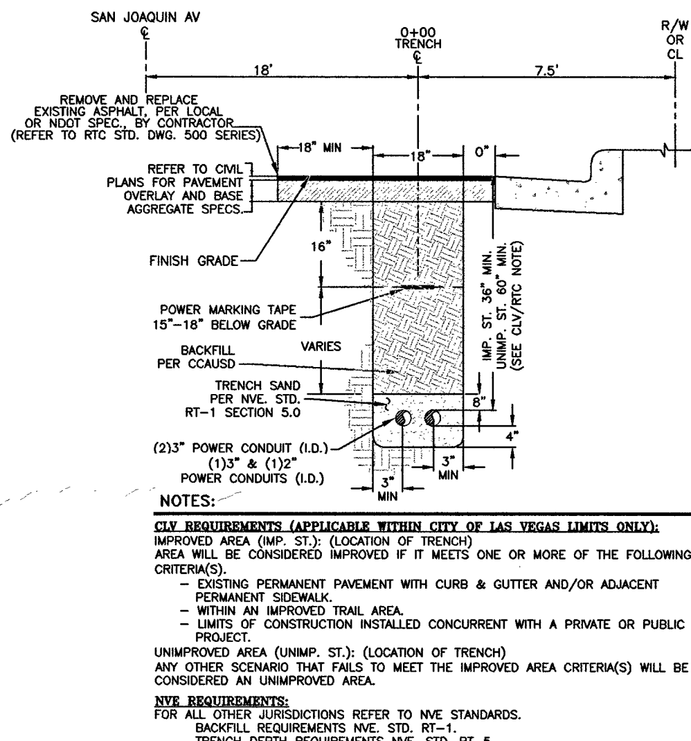
TRENCH DETAIL SECTION "A"
