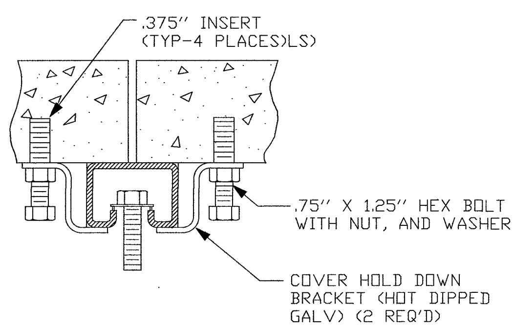
DETAIL "A-4"
