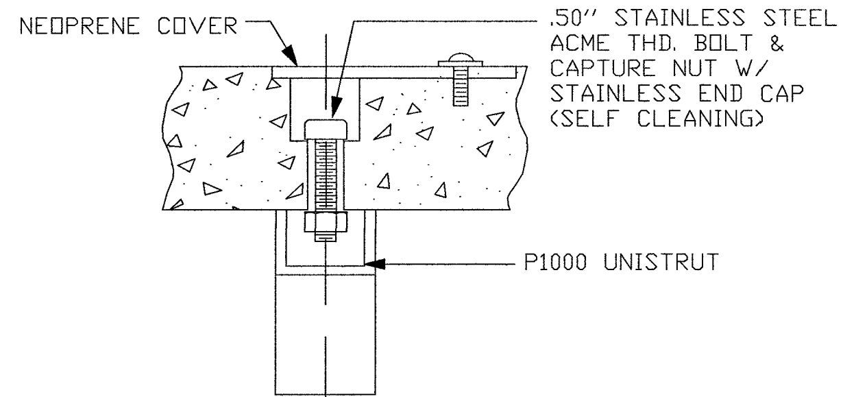
DETAIL "A-3"
