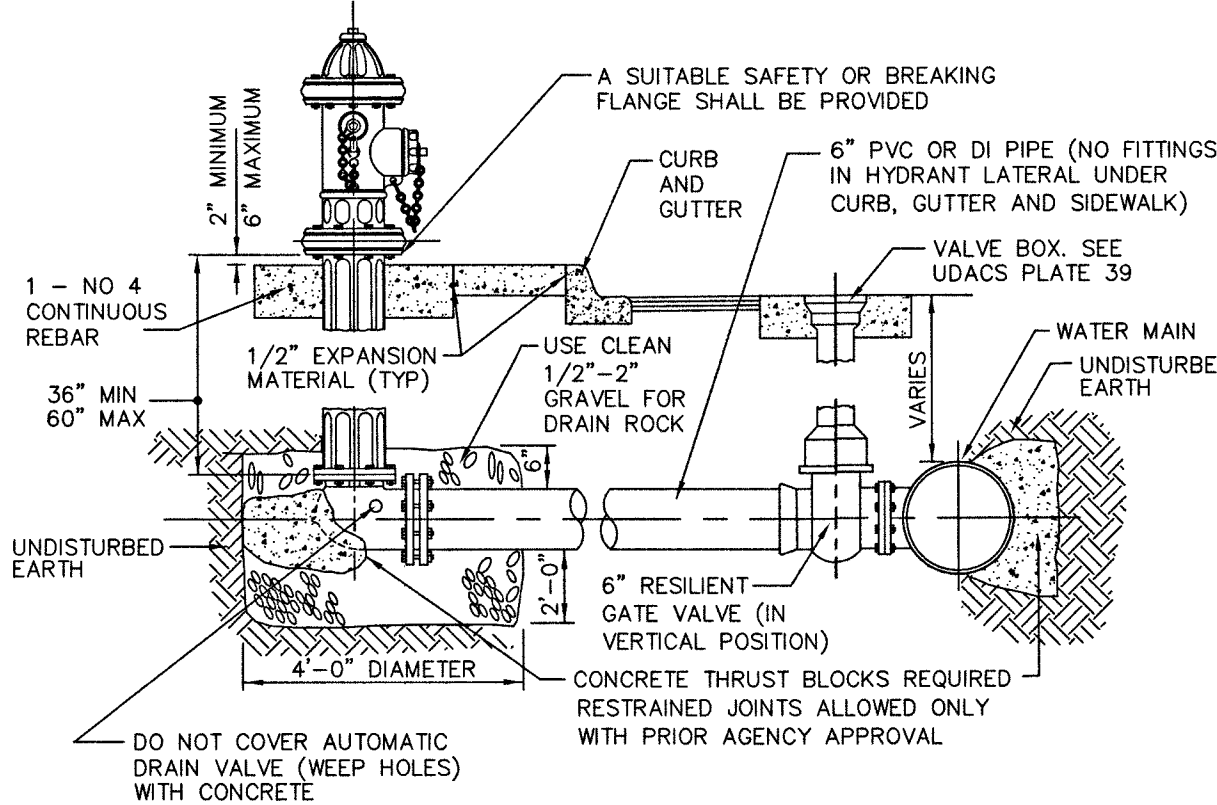
HYDRANT ASSEMBLY DETAIL
