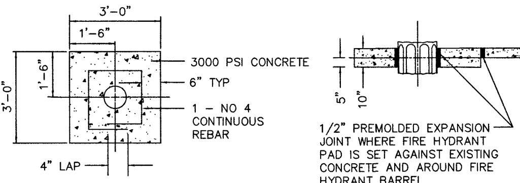
PAD DETAIL
