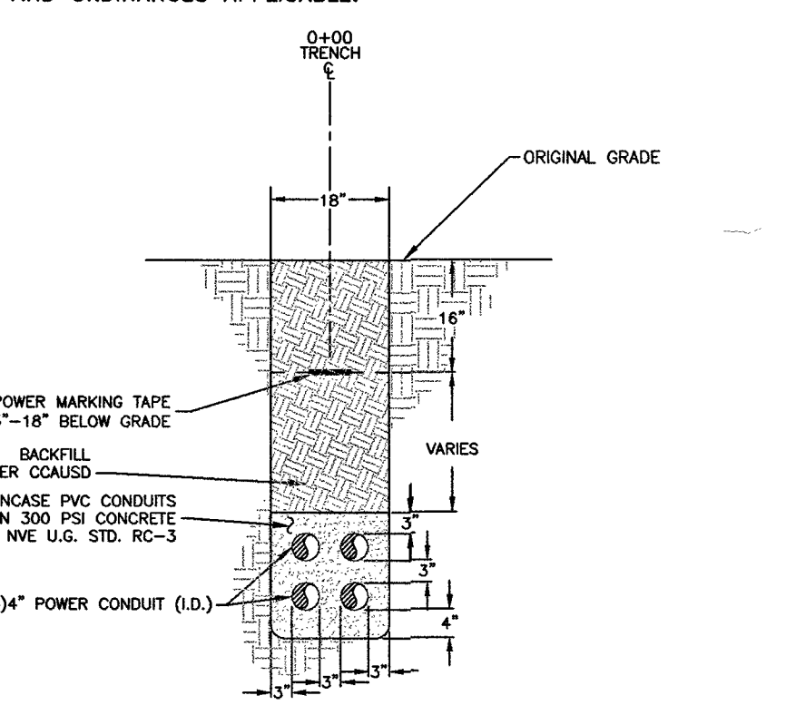
TRENCH DETAIL SECTION "C"
