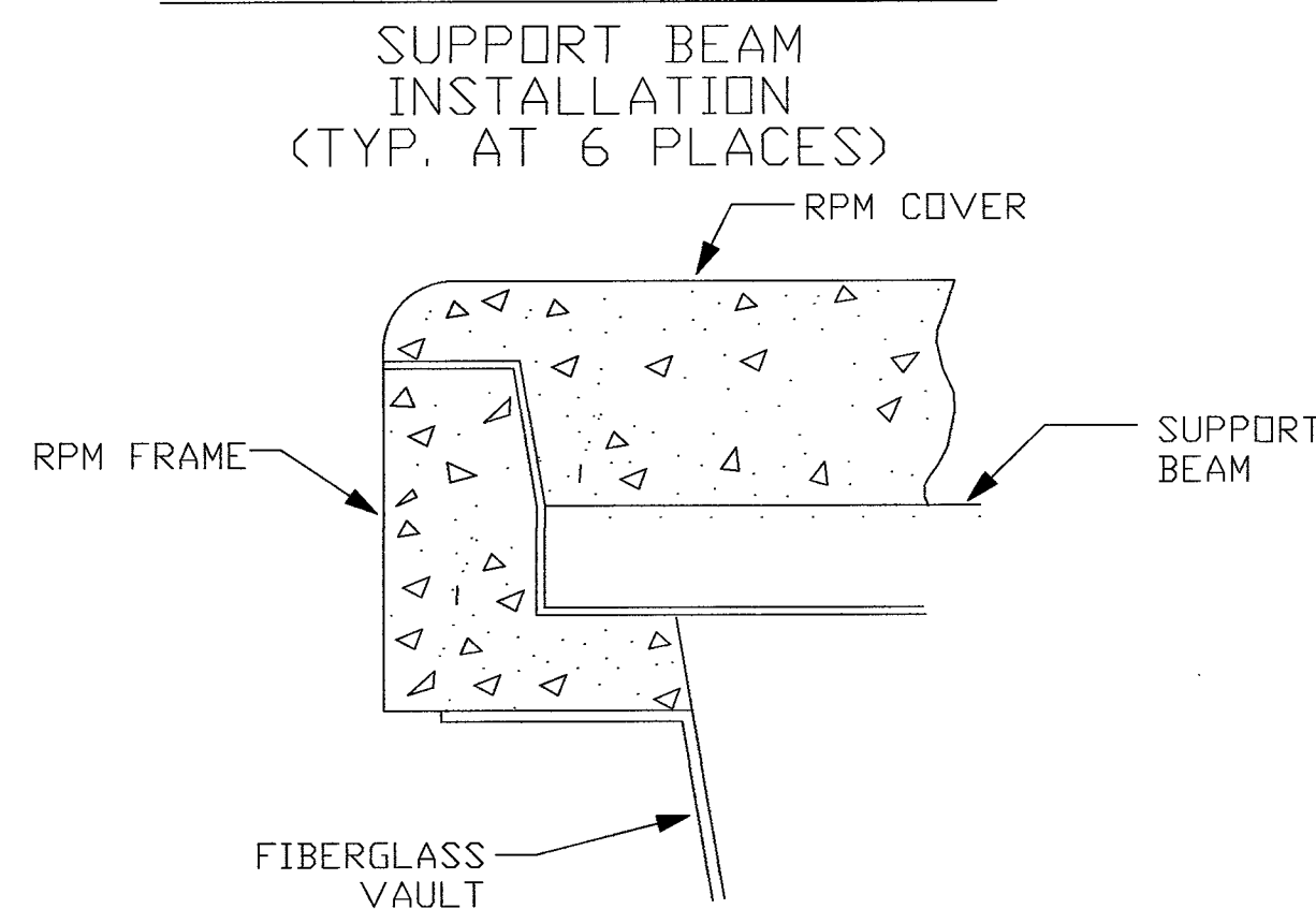
DETAIL "A-4"
