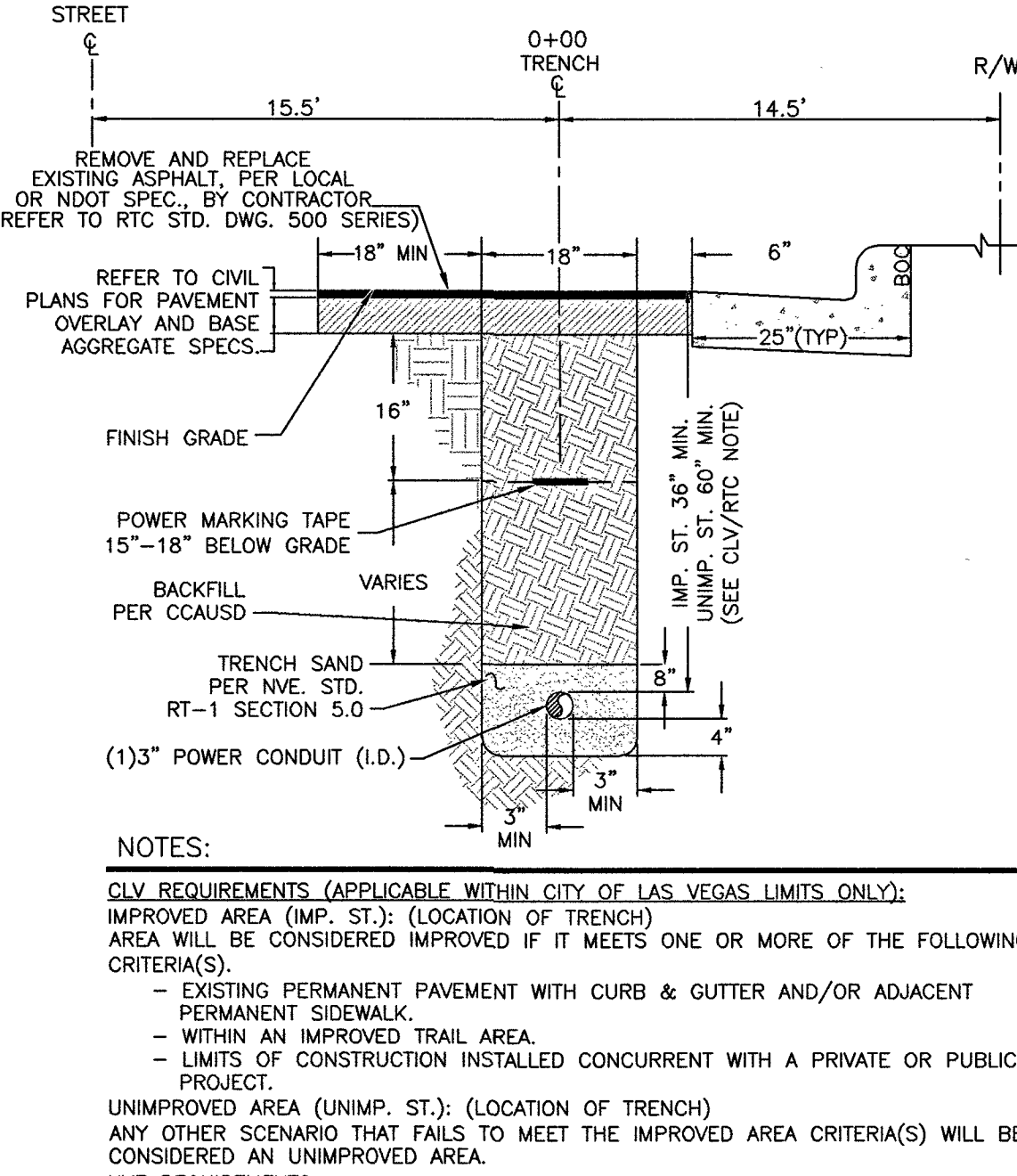
TRENCH DETAIL 1-3\"/>
