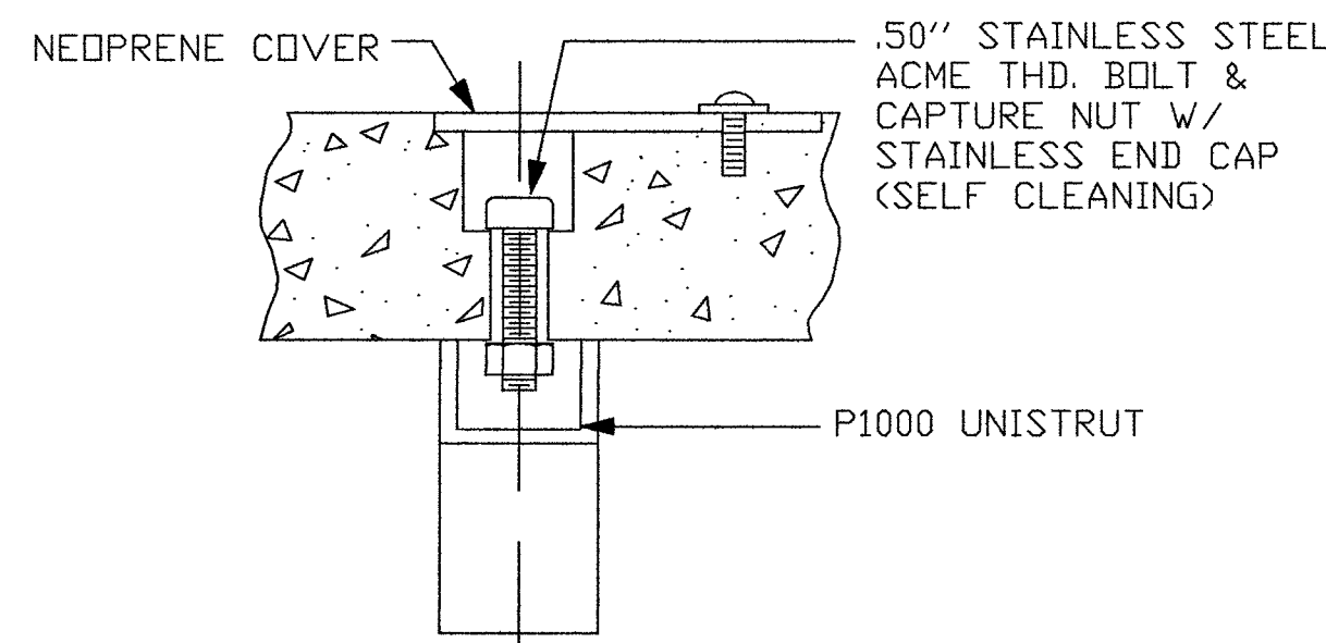
DETAIL "A-3"
