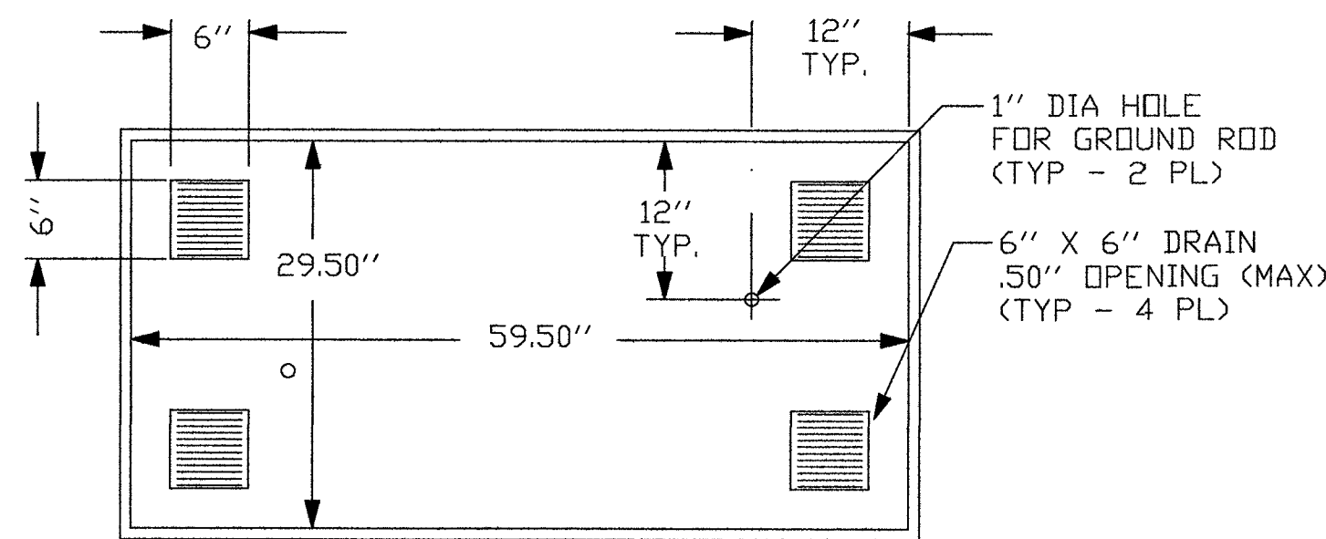
DETAIL "D"
