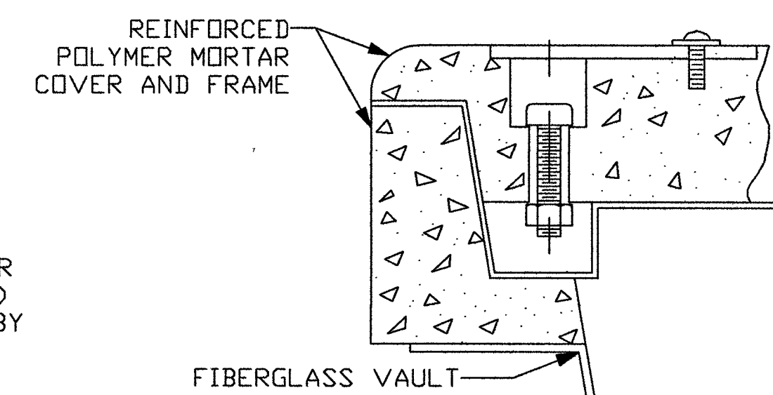
SECTION A-A LOCKING DEVICE CROSS SECTION
