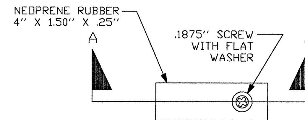
DETAIL "A-1" LOCK DOWN DEVICE
