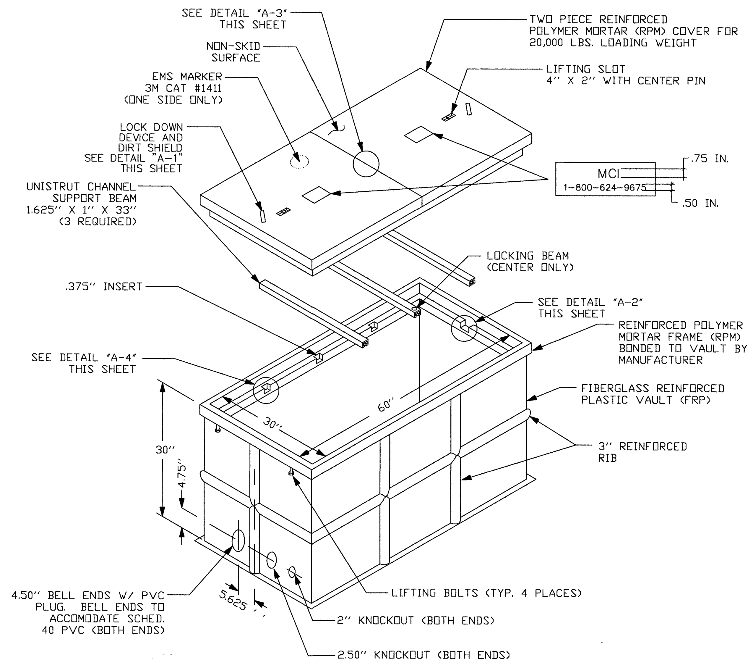
DETAIL "A" EXPLODED ISOMETRIC DETAIL
