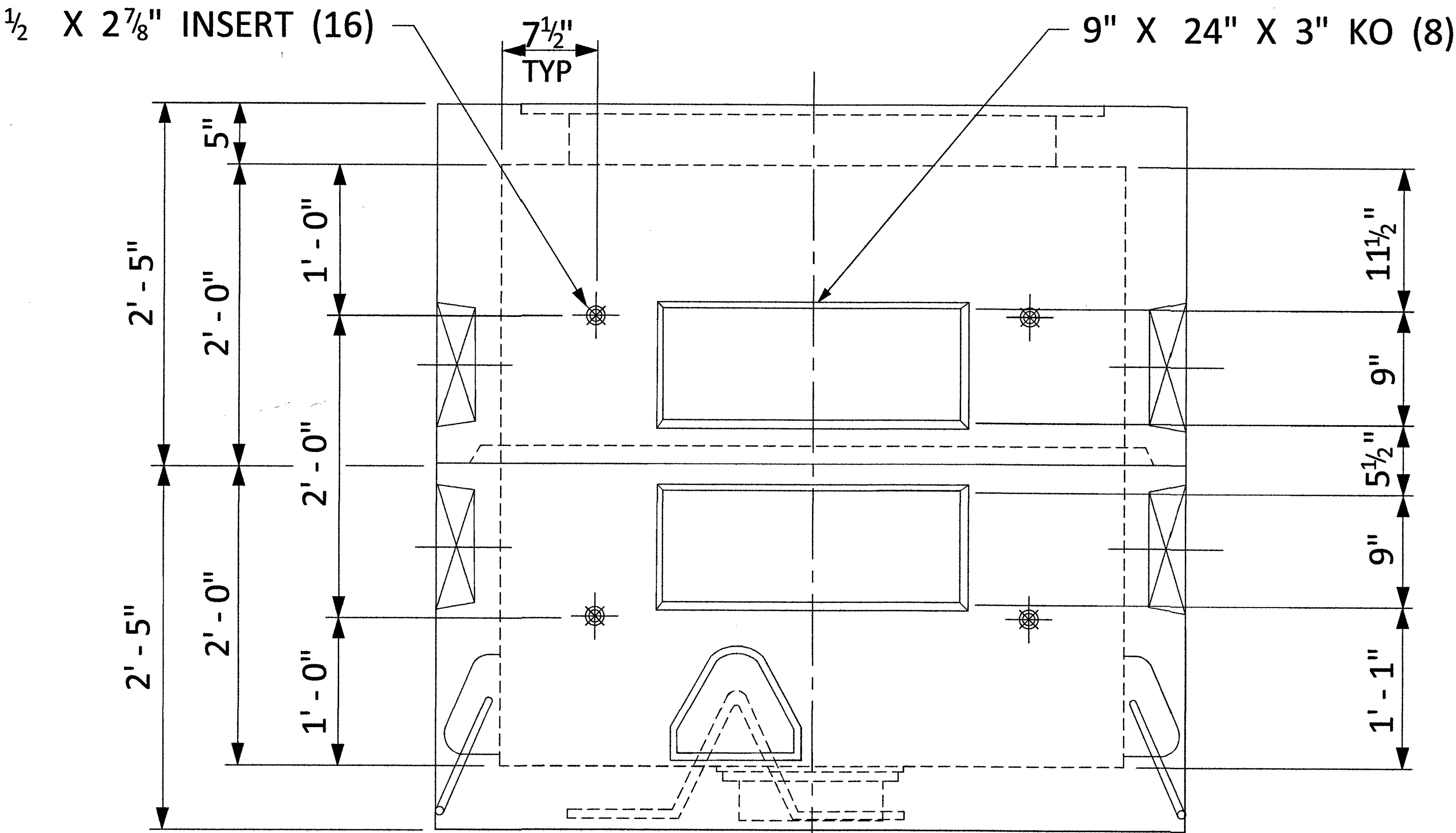
VIEW A, B, C, D SCALE: 1/2" = 1'-0"
