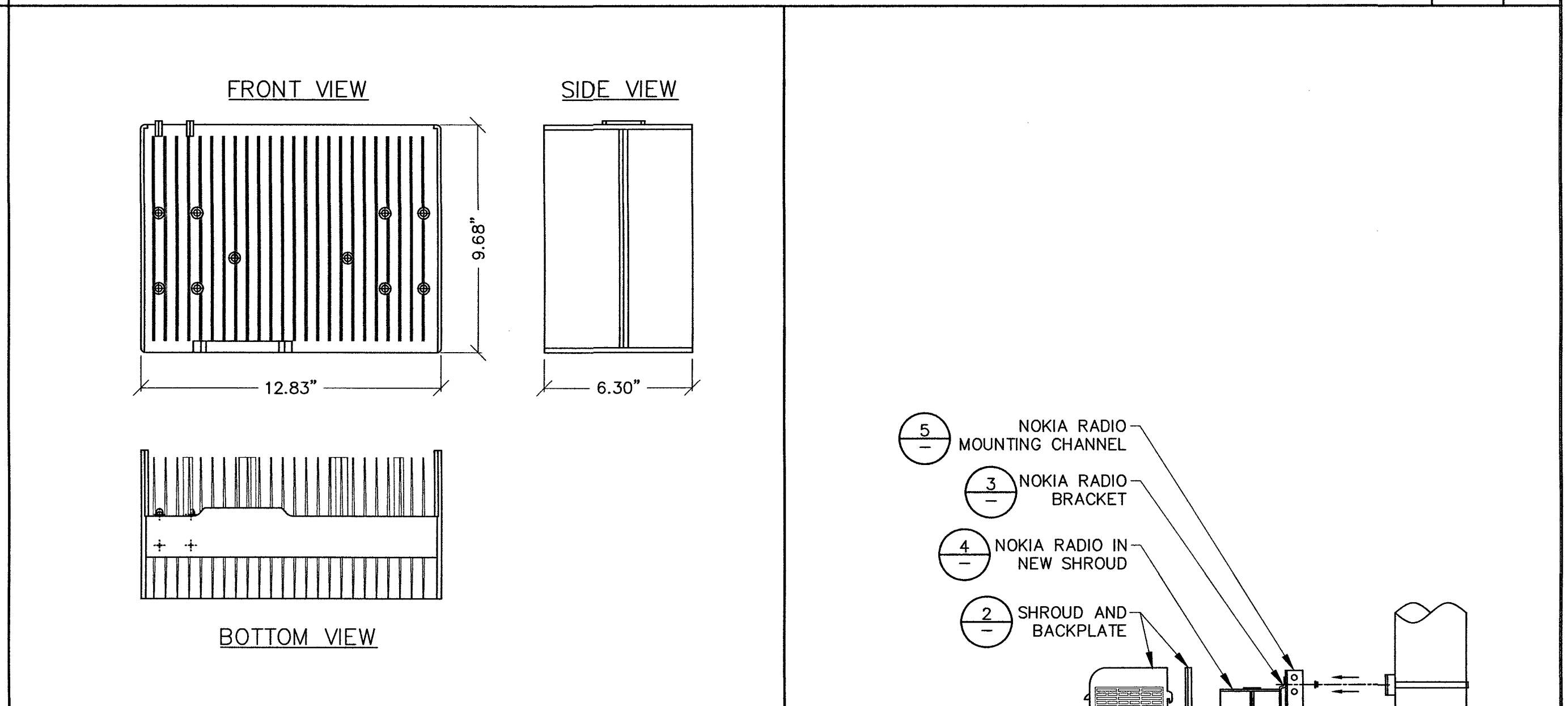
7 RADIO SHROUD
