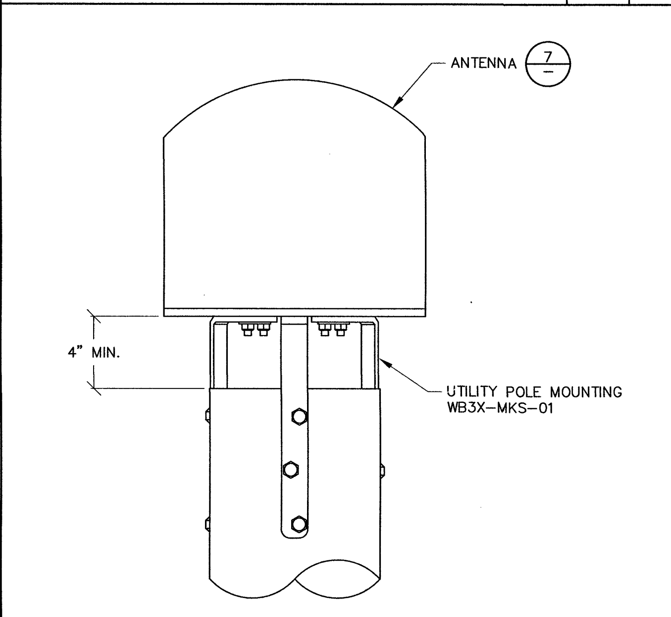
9 ANTENNA DETAIL
