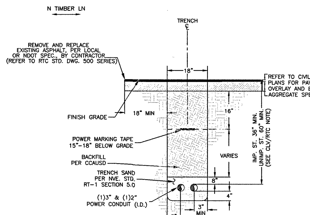
TRENCH DETAIL SECTION "A"
