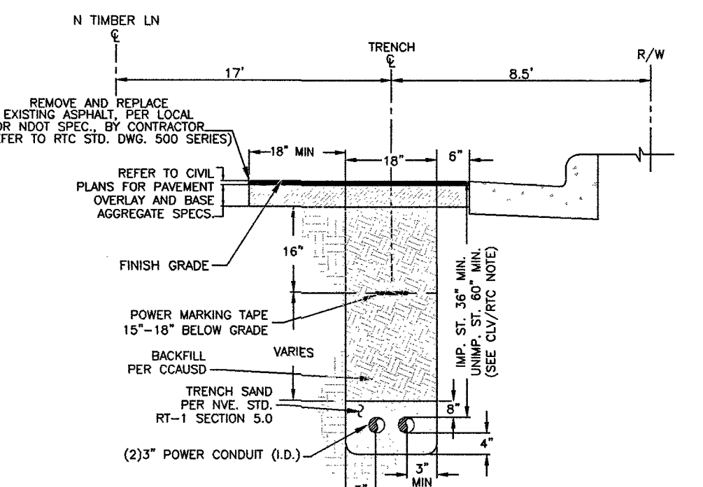
TRENCH DETAIL SECTION "B"
