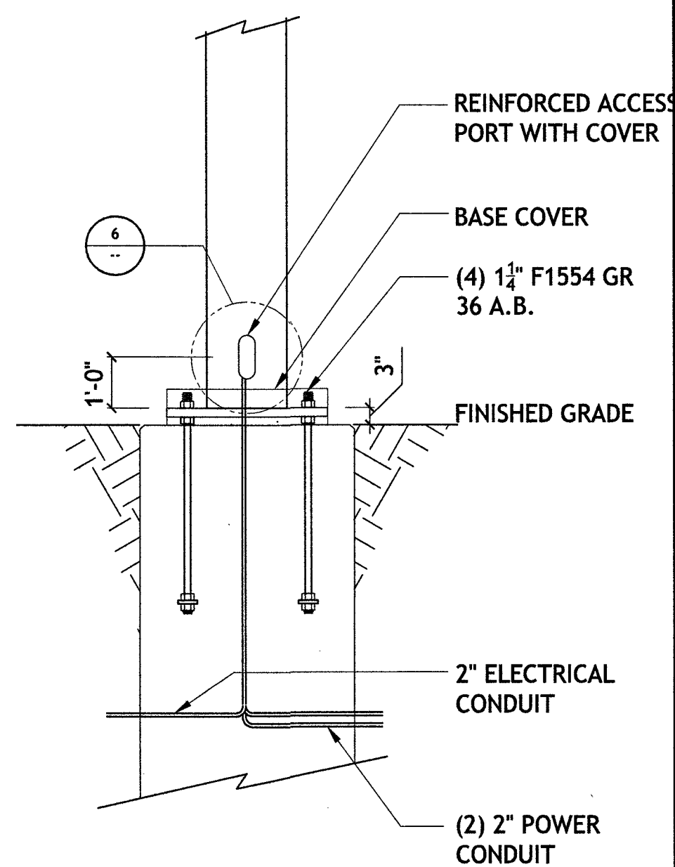
5 BASE DETAIL
