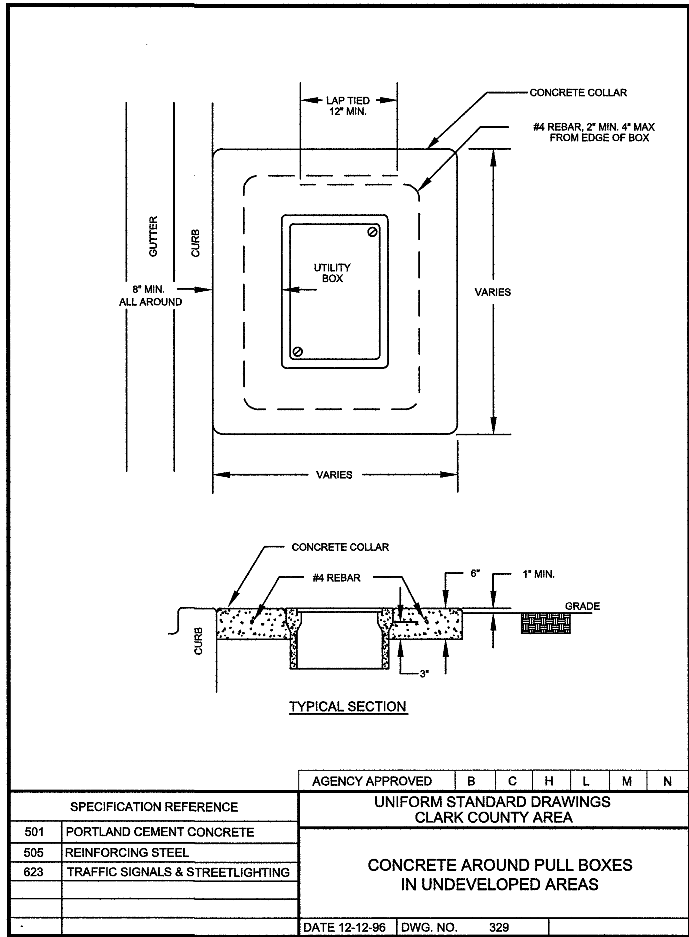
PULL BOX INSTALLATION DETAIL
