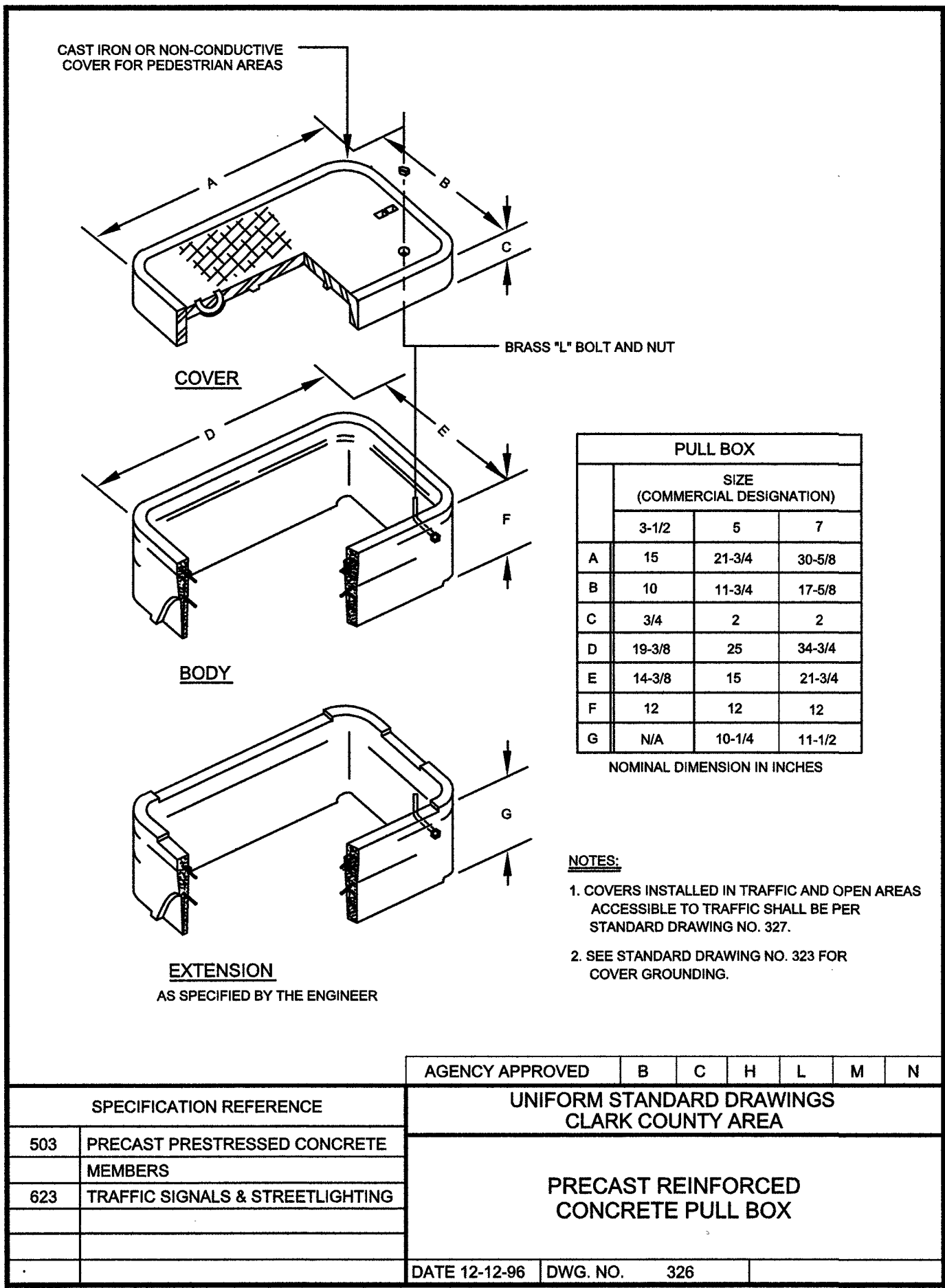
CONCRETE PULL BOX SPECIFICATIONS
