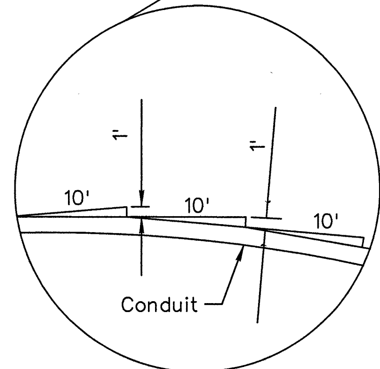
TYPICAL VERTICAL ROUTING OF CONDUIT UNDER AN OBSTRUCTION
