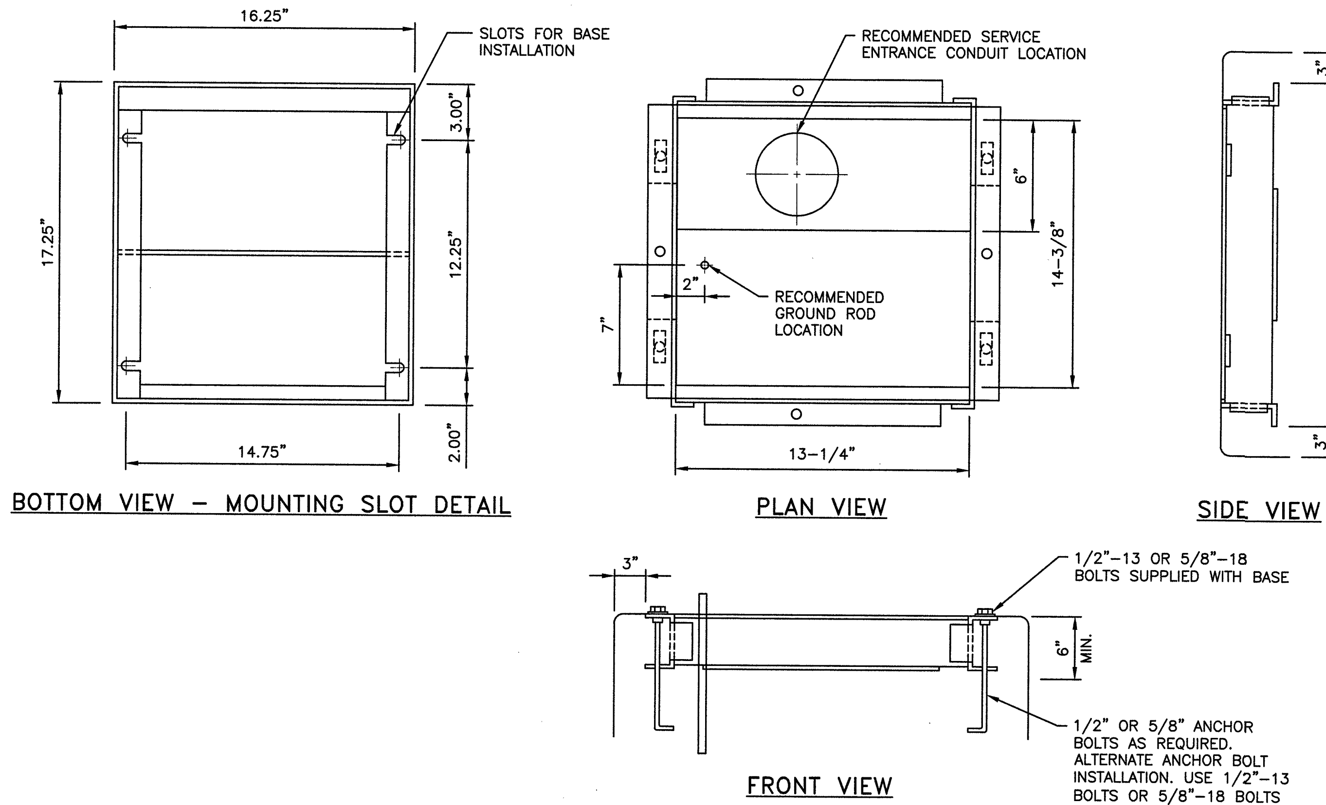
BASEPLATE DETAIL
