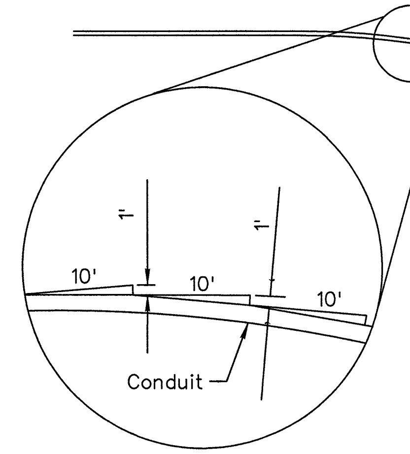
TYPICAL HORIZONTAL ROUTING OF CONDUIT AROUND AN OBSTRUCTION
