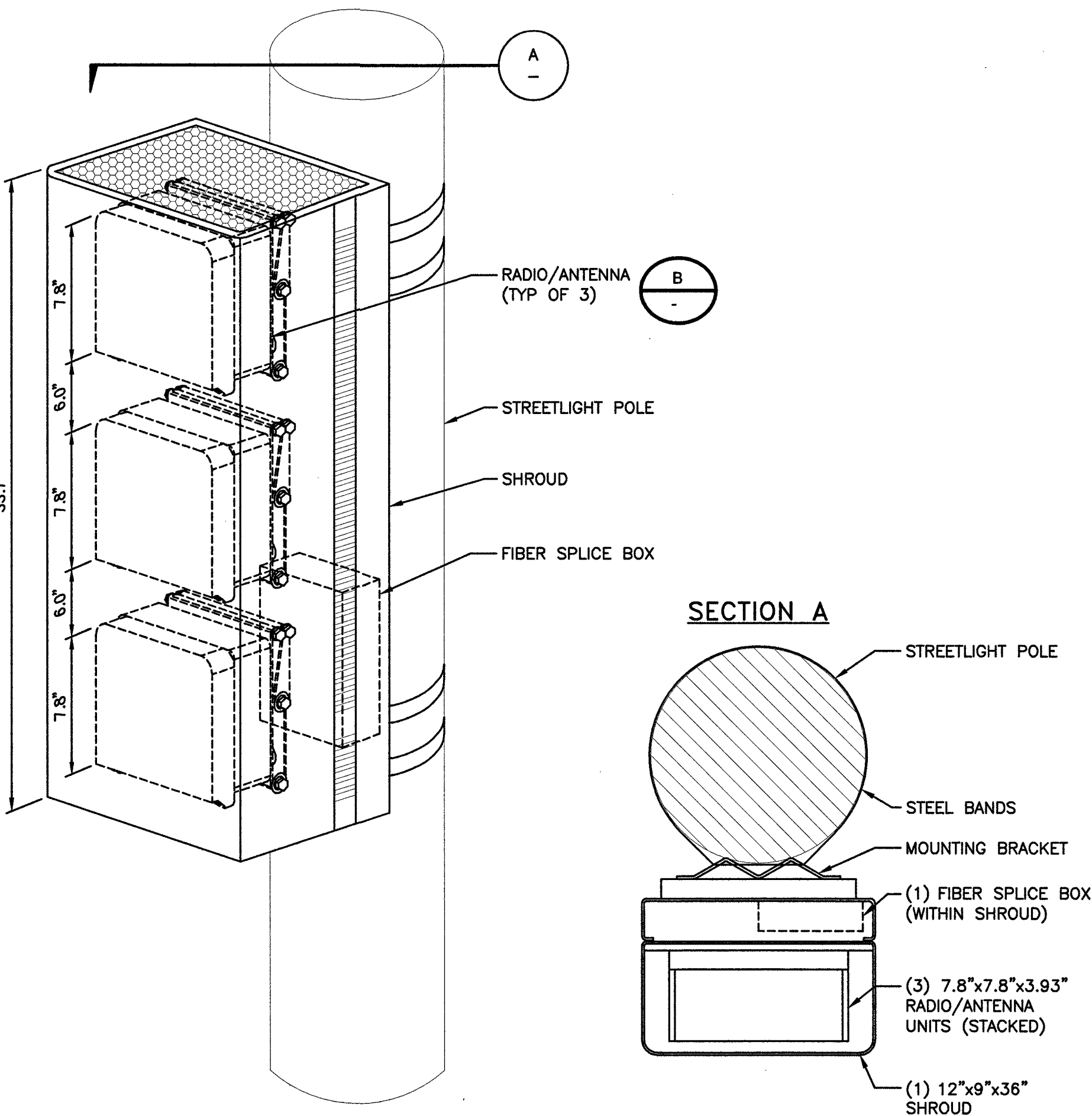
RADIO SHROUD MOUNTING DETAIL
