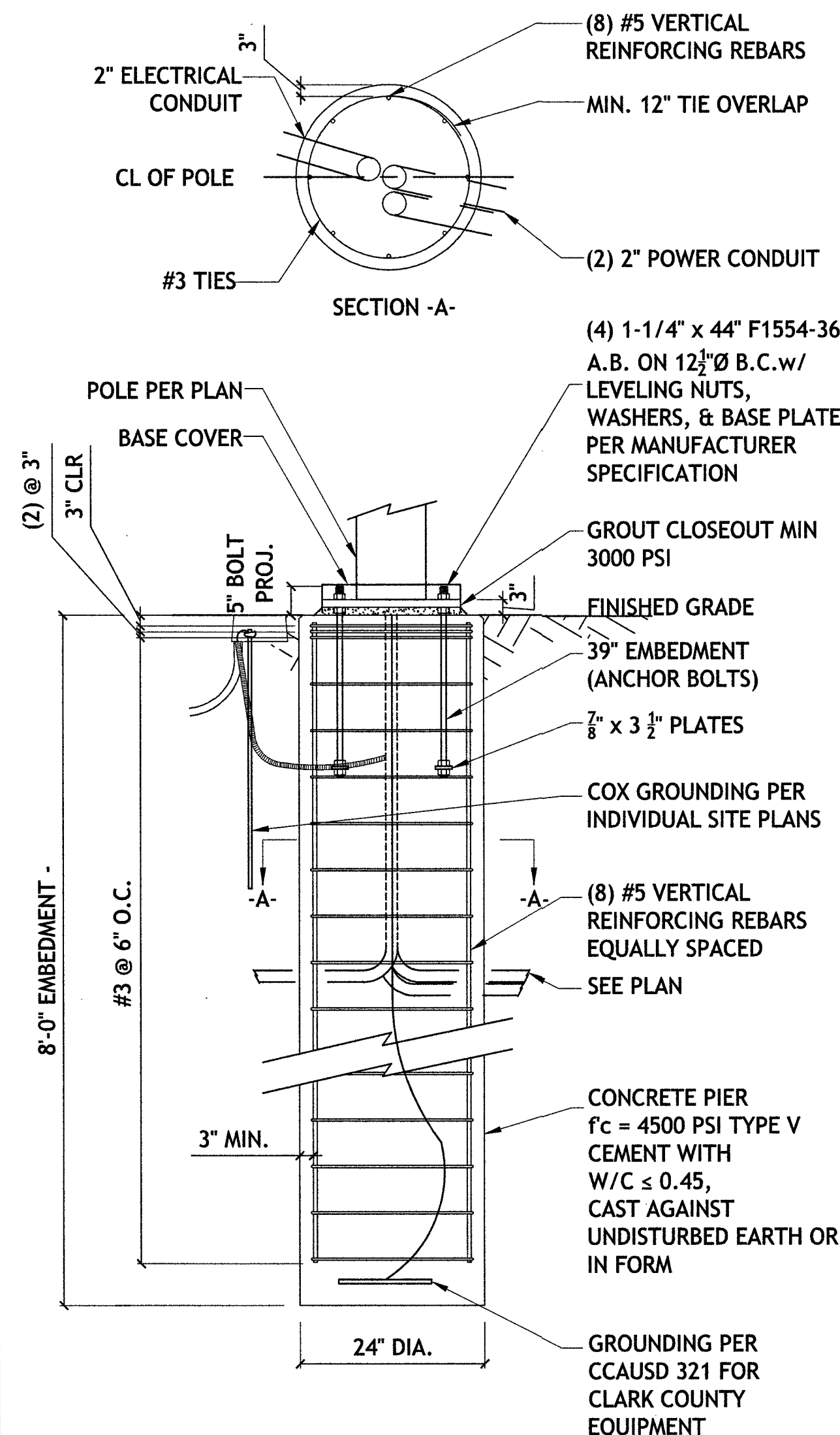
2 PIER FOUNDATION
