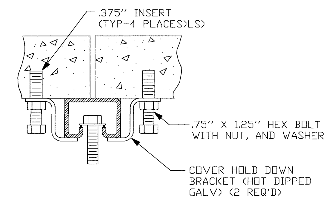
DETAIL "A-4"
