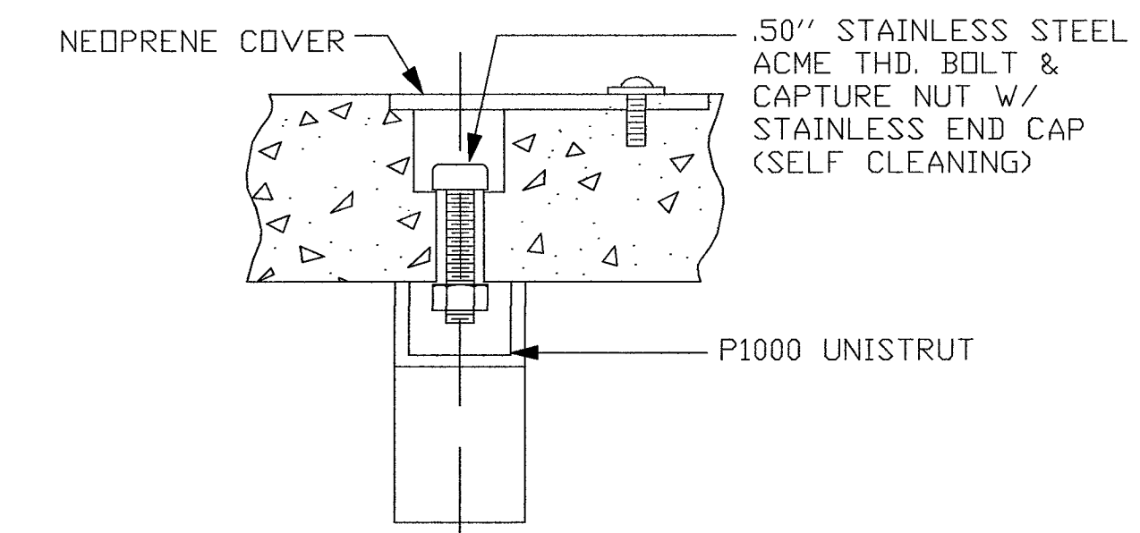
DETAIL "A-3"
