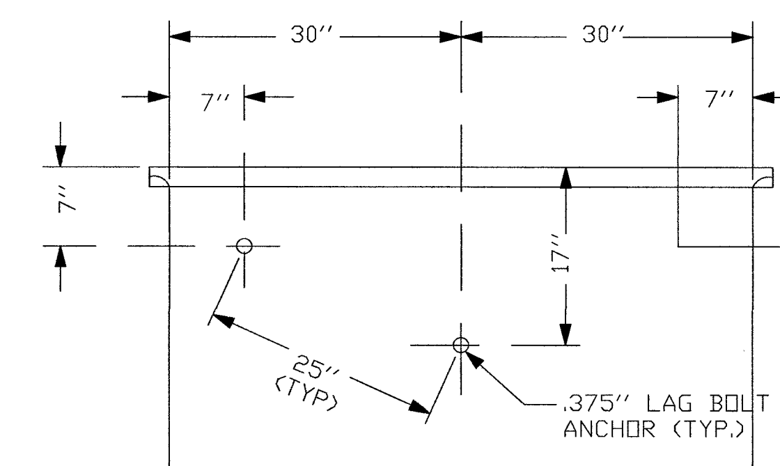
SIDE WALL VIEW INSIDE LOOKING OUT
