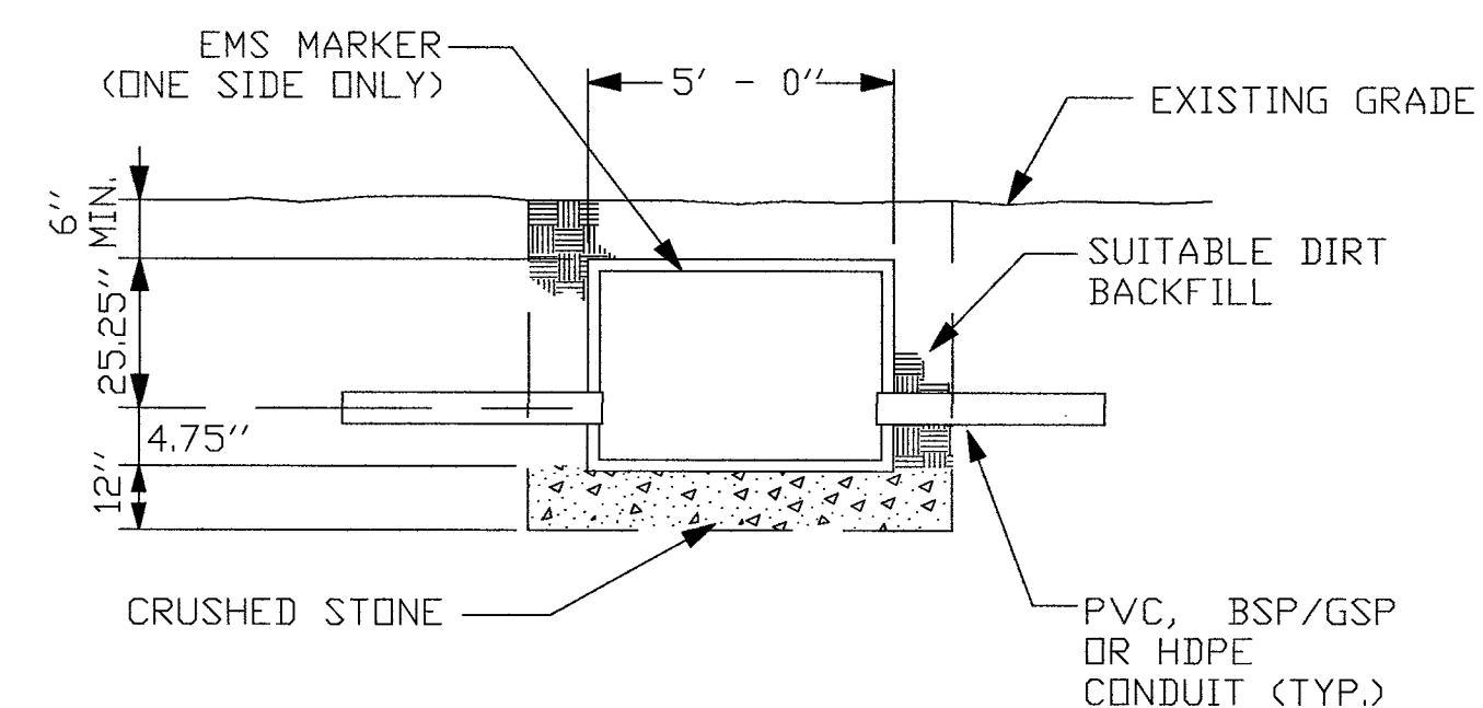
PROFILE
