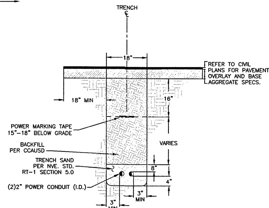
TRENCH DETAIL SECTION "A"
