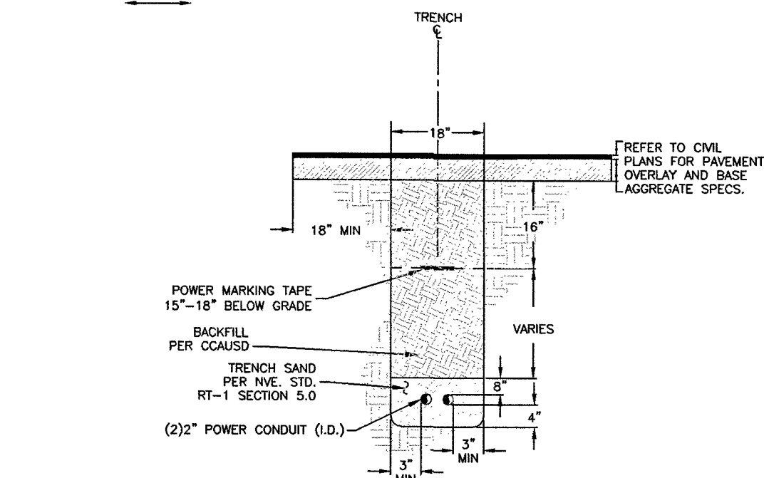
TRENCH DETAIL SECTION "A"
