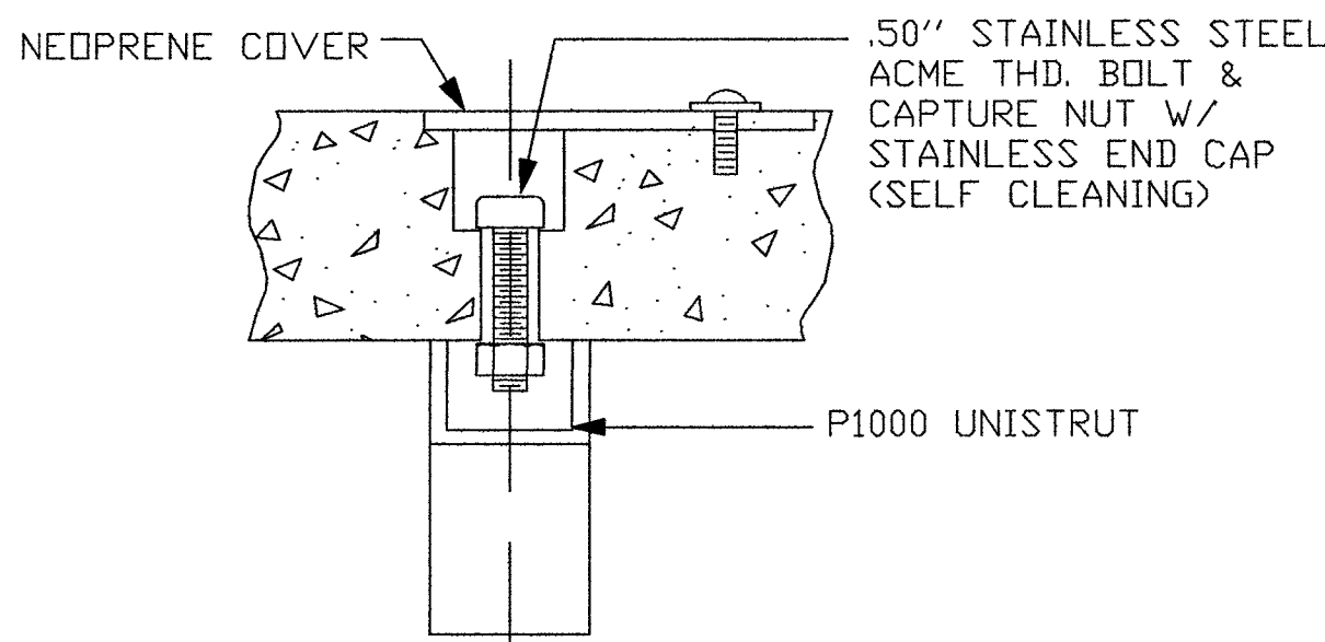
DETAIL "A-3"
