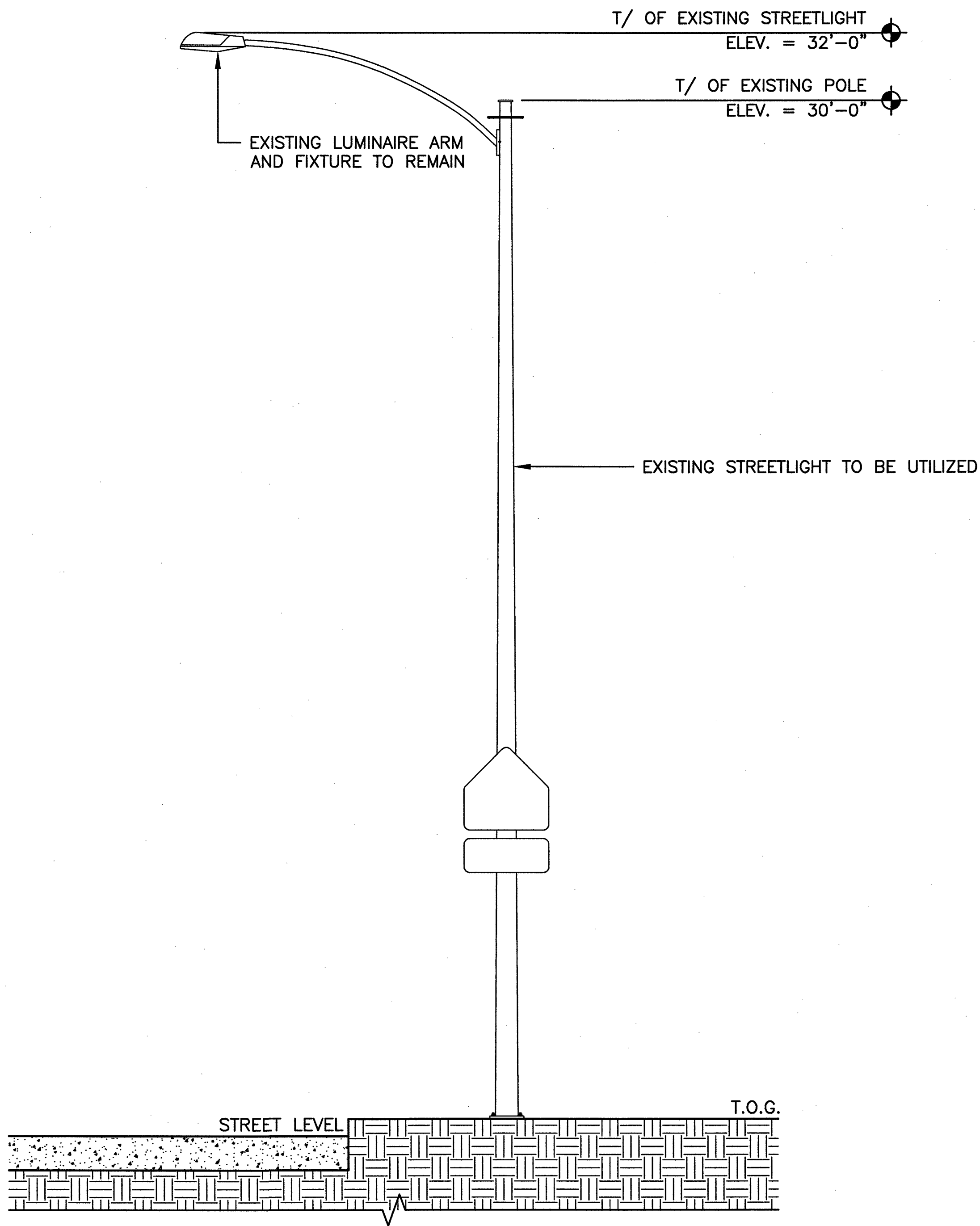
1 EXISTING POLE ELEVATION SCALE: 0' 1' 4' 8' 16'
