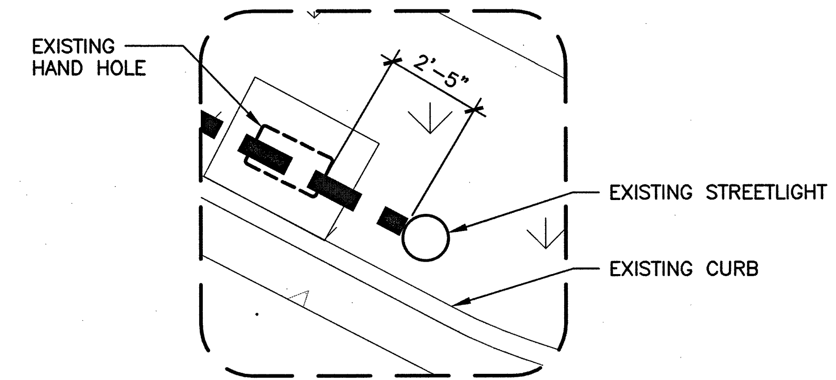
3 HAND HOLE PLACEMENT SCALE: 0' 1' 4' 8' 16'
