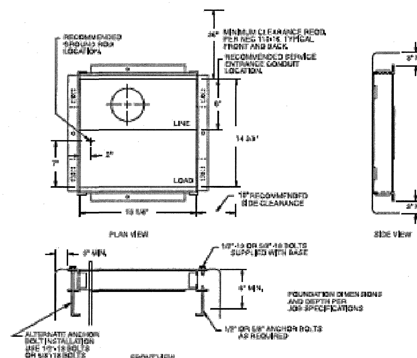
BASE DETAIL
