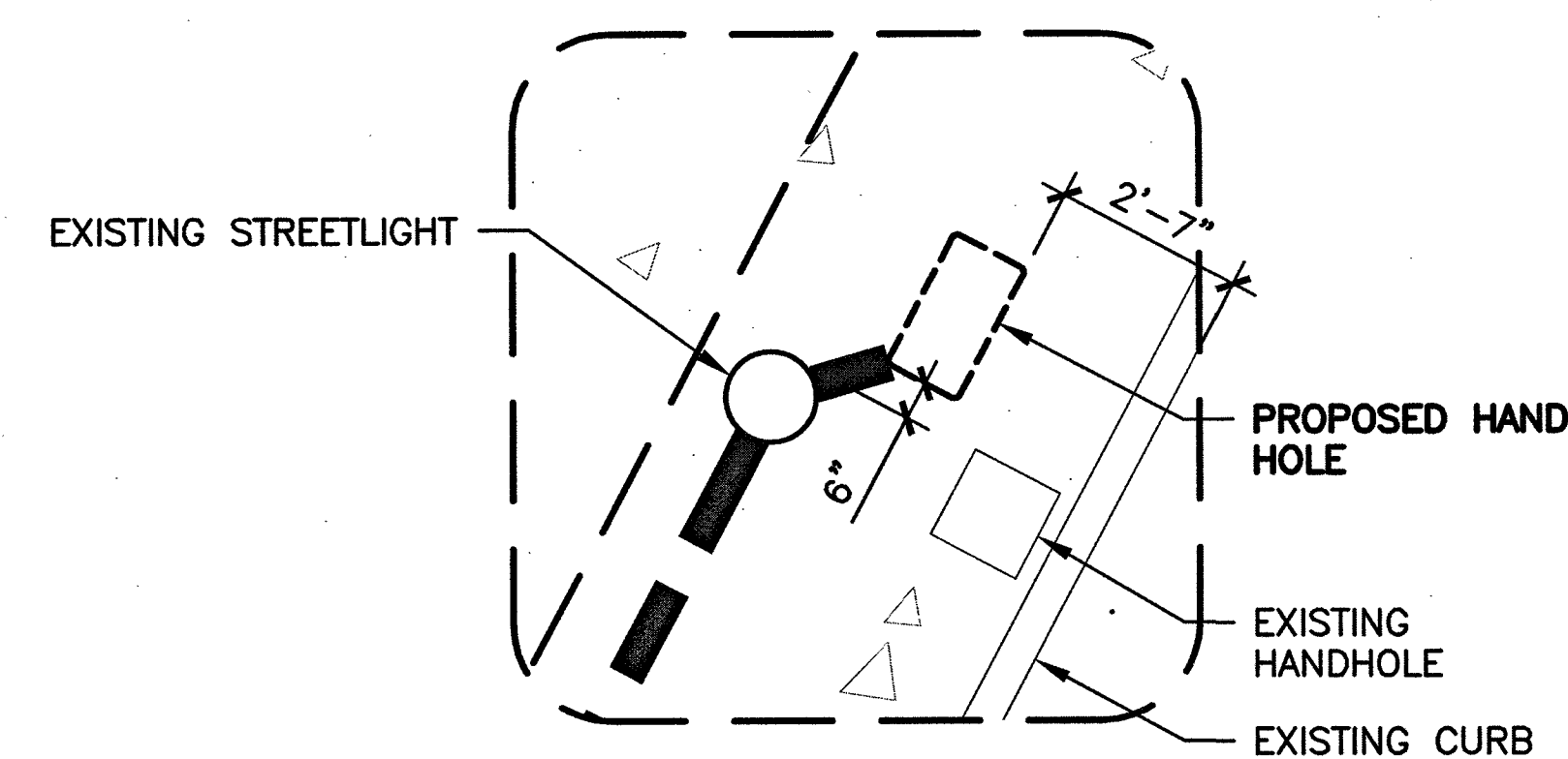
3 HAND HOLE PLACEMENT
