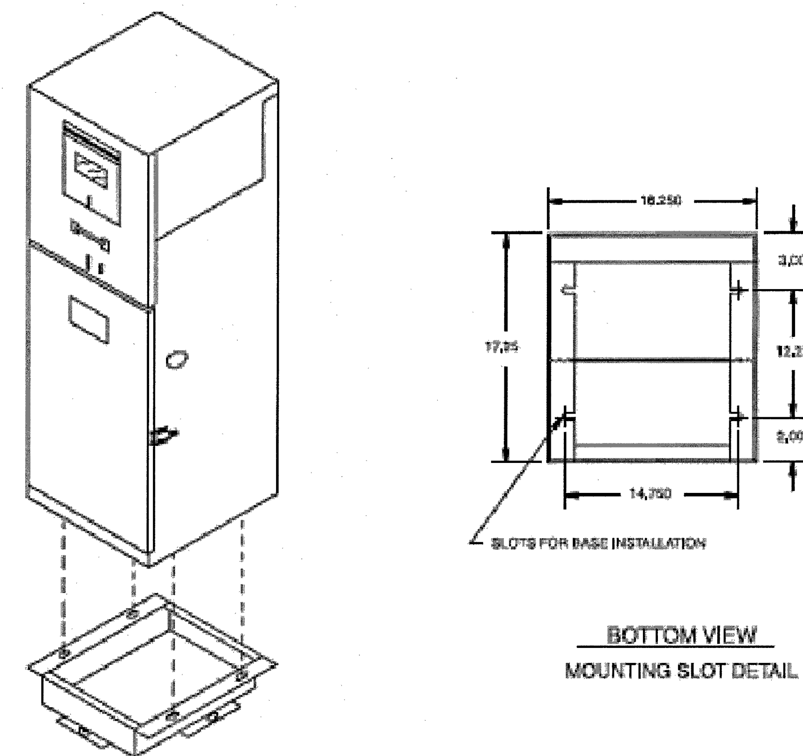
BASE DETAIL
