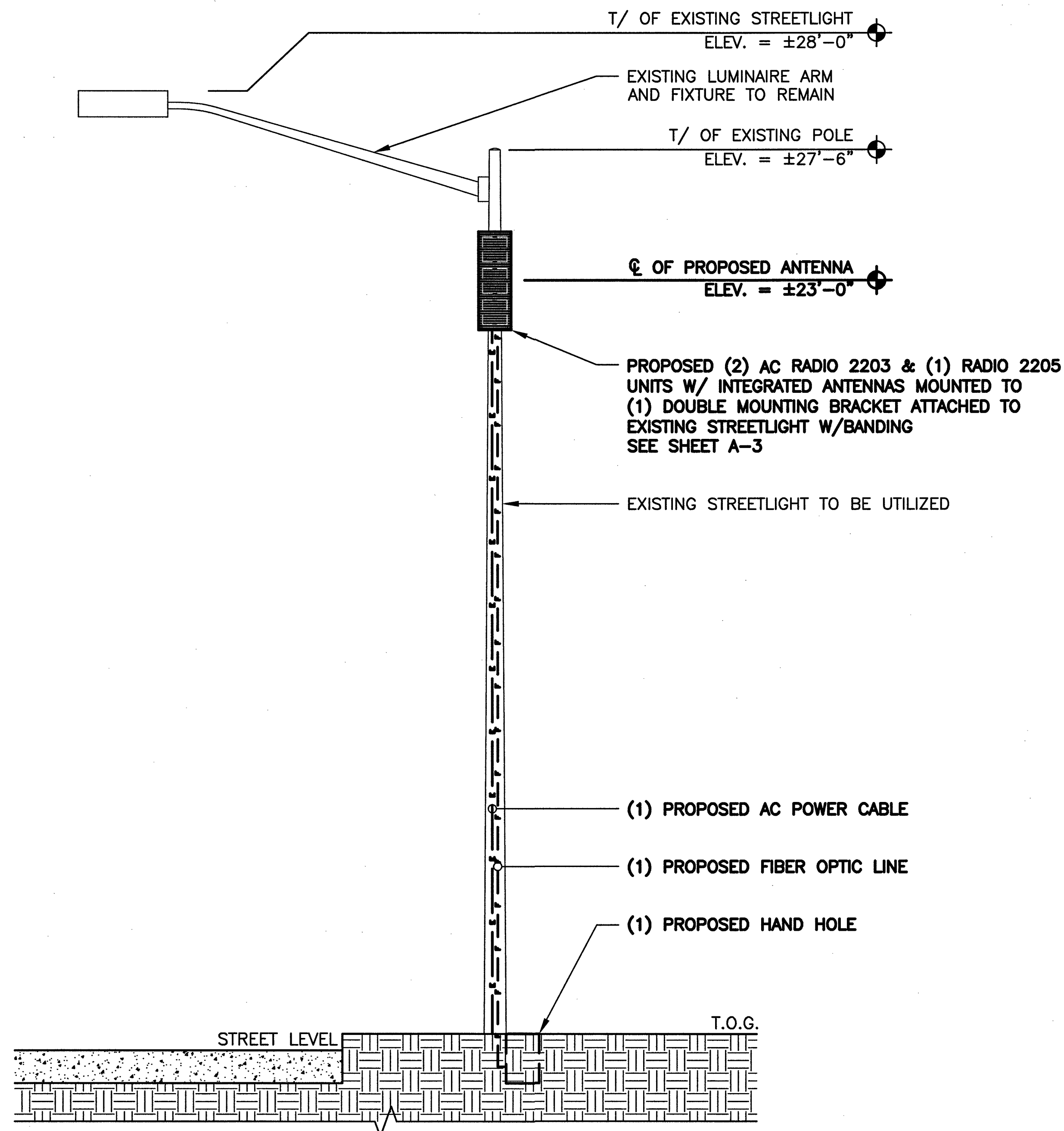
2 FINAL POLE ELEVATION SCALE: 0' 1' 4' 8' 16'
