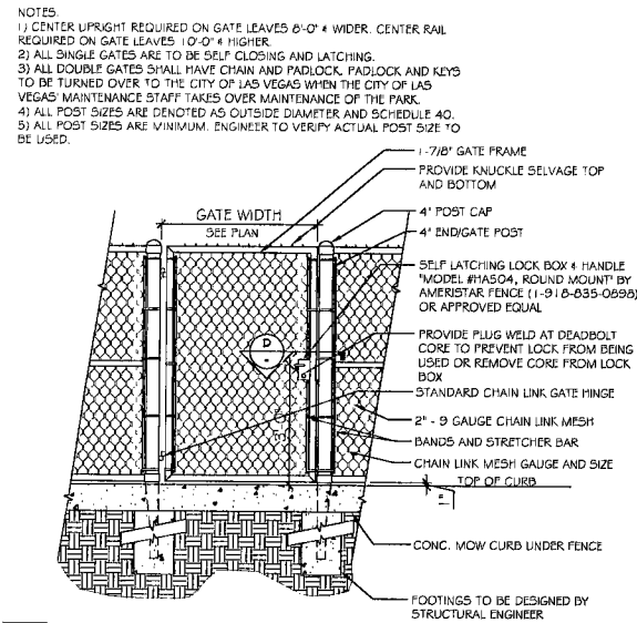
A CHAIN LINK FENCE GATE ELEVATION
