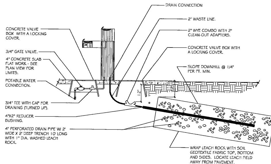
H DRINKING FOUNTAIN DETAIL WITH DRAIN FIELD
