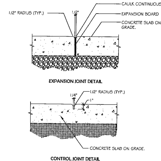
G CONTROL & EXPANSION JOINT DETAILS
