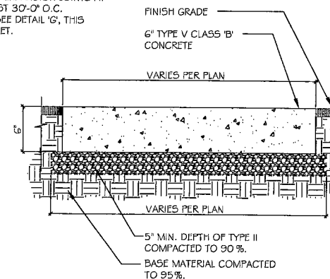
F SIDEWALK DETAIL
