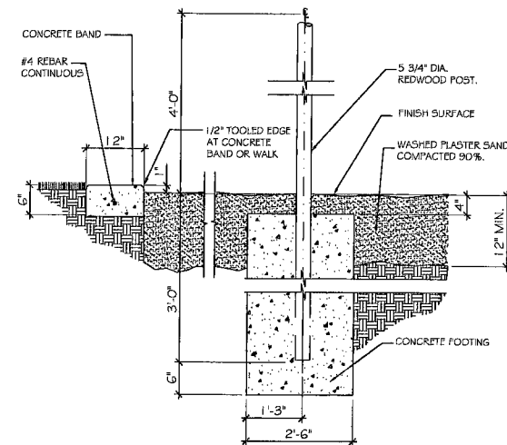
E MARKING POST
