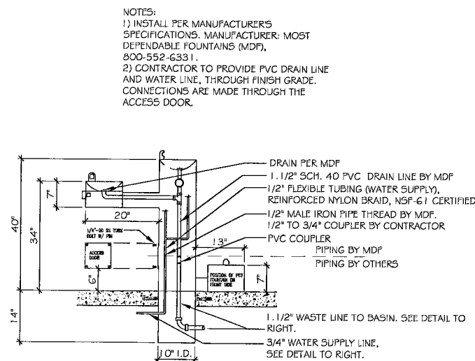
H DRINKING FOUNTAIN DETAIL WITH DRAIN FIELD
