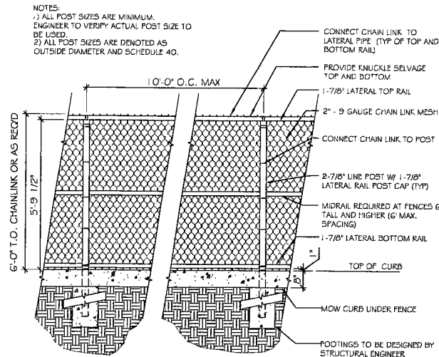
B CHAIN LINK FENCE ELEVATION
