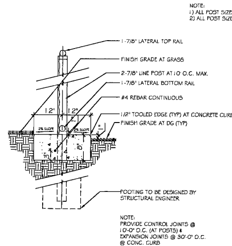
C CHAIN LINK FENCE SECTION
