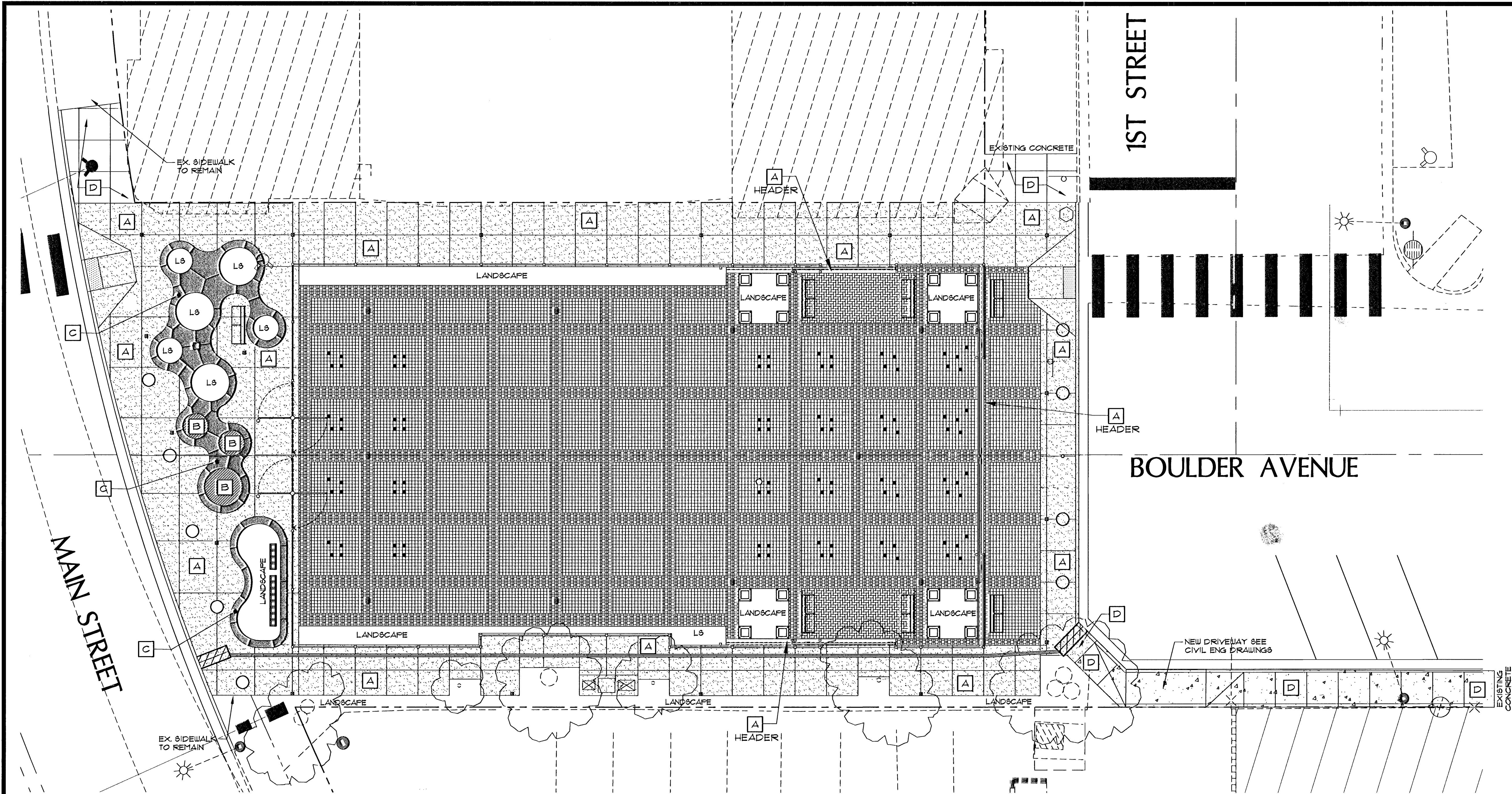
1 DECORATIVE ARCHITECTURAL CONCRETE PLAN BASE SCALE: 1/8" = 1'-0"
