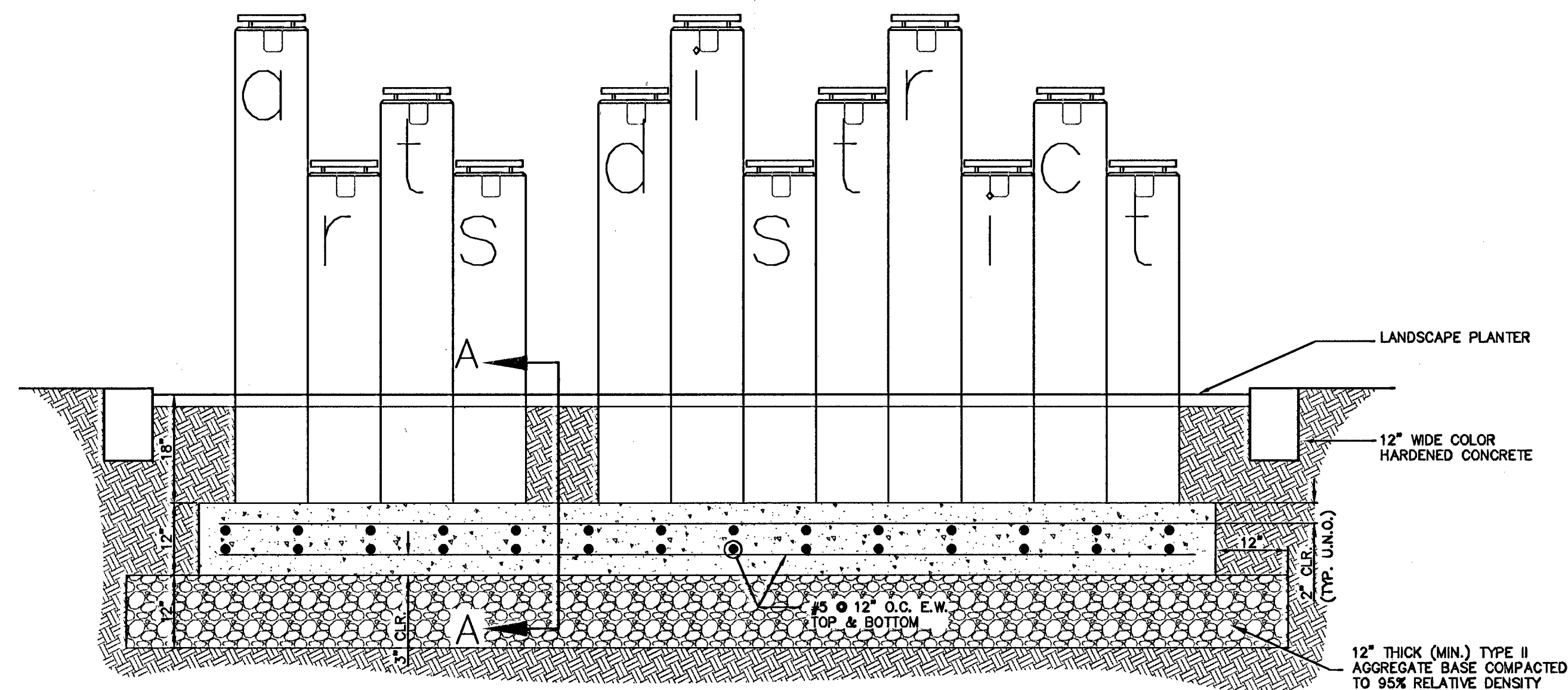
MONUMENT FOOTING DETAIL N.T.S.
