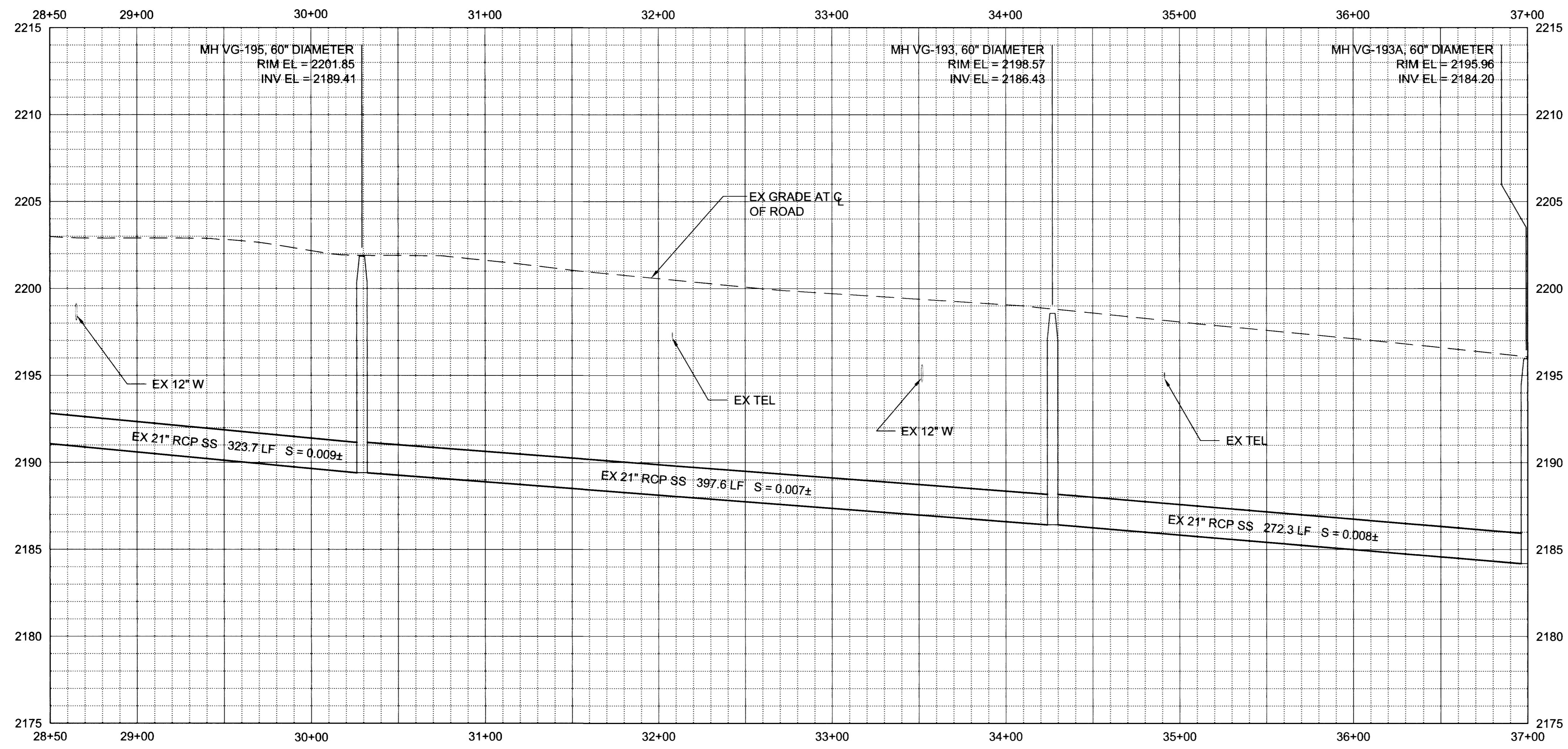
VEGAS DRIVE PROFILE SCALE: HORIZ 1" = 40' VERT 1" = 4'
