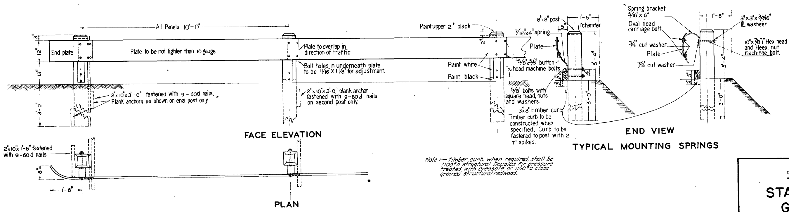
TYPICAL BEAM TYPE GUARD RAIL
