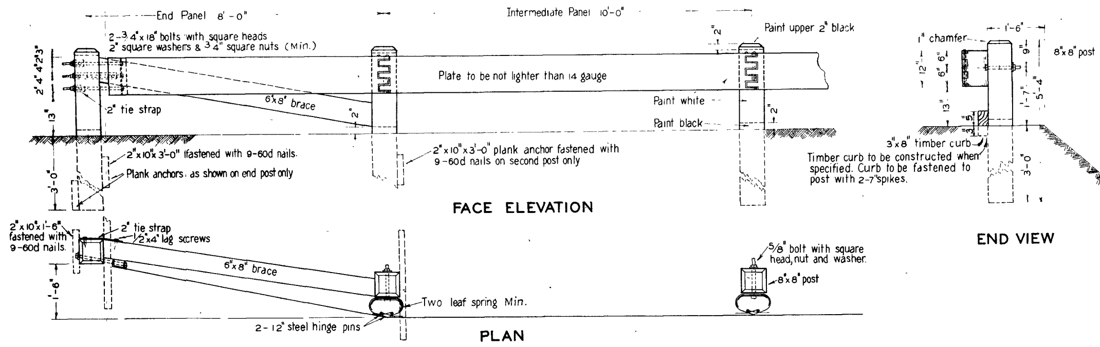
TYPICAL FLOATING TYPE GUARD RAIL
